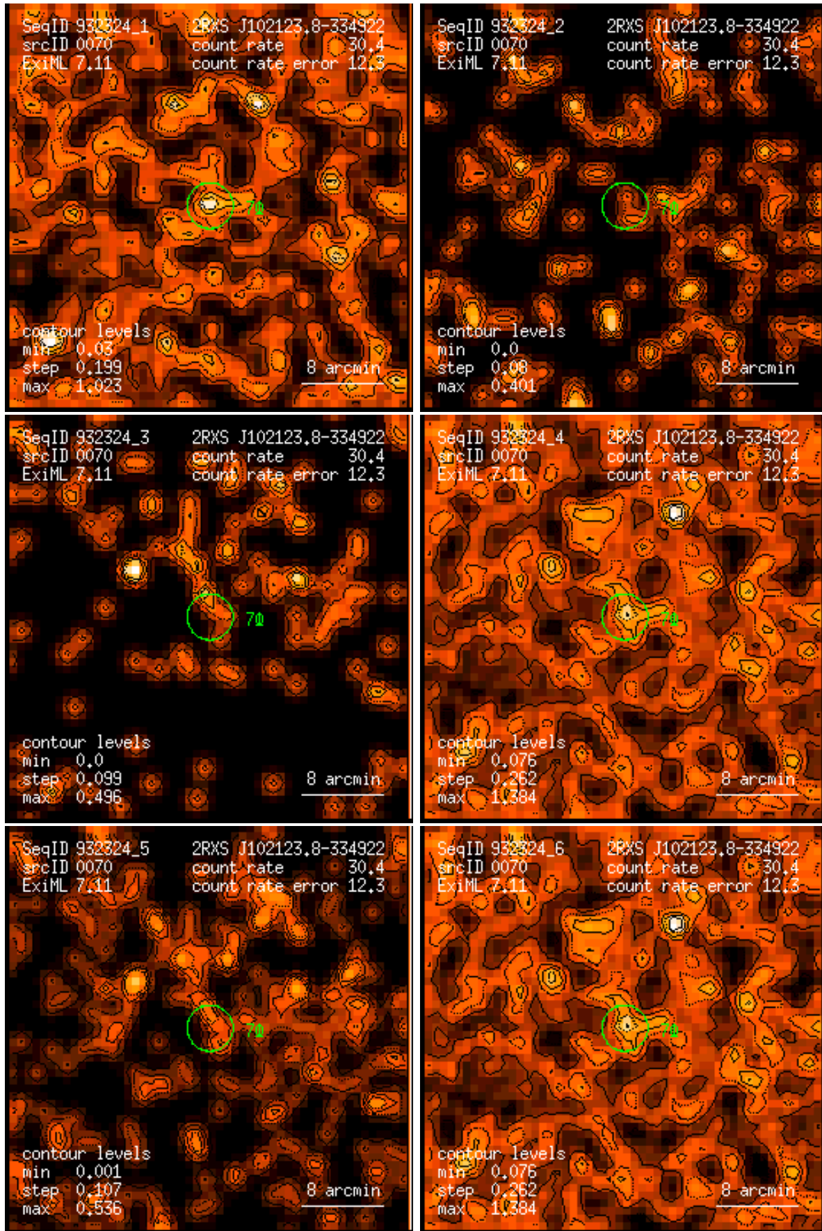
Figure 70: RASS 932324: detection 0070: band rate images, Gaussian filter: (1) PSPC channels 11 – 41, (2) 52 – 90, (3) 91 – 201, (4) 11 – 235, (5) 52 – 201, (6) 11 – 201. Broad band rates in counts/ks. Band rate contour levels in counts/ks/arcmin 2 .
