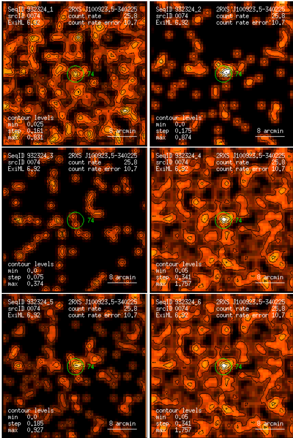
Figure 74: RASS 932324: detection 0074: band rate images, Gaussian filter: (1) PSPC channels 11 – 41, (2) 52 – 90, (3) 91 – 201, (4) 11 – 235, (5) 52 – 201, (6) 11 – 201. Broad band rates in counts/ks. Band rate contour levels in counts/ks/arcmin 2 .
