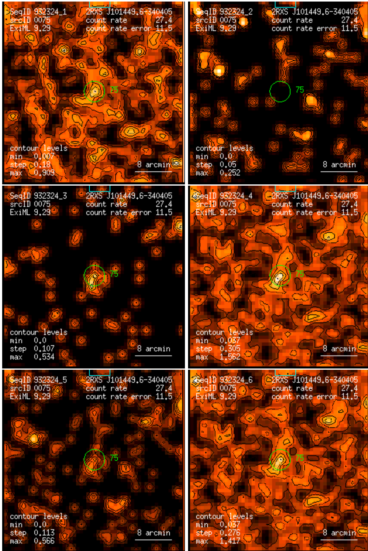
Figure 75: RASS 932324: detection 0075: band rate images, Gaussian filter: (1) PSPC channels 11 – 41, (2) 52 – 90, (3) 91 – 201, (4) 11 – 235, (5) 52 – 201, (6) 11 – 201. Broad band rates in counts/ks. Band rate contour levels in counts/ks/arcmin 2 .
