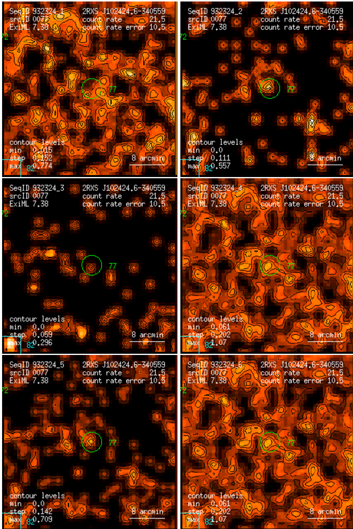
Figure 77: RASS 932324: detection 0077: band rate images, Gaussian filter: (1) PSPC channels 11 – 41, (2) 52 – 90, (3) 91 – 201, (4) 11 – 235, (5) 52 – 201, (6) 11 – 201. Broad band rates in counts/ks. Band rate contour levels in counts/ks/arcmin 2 .
