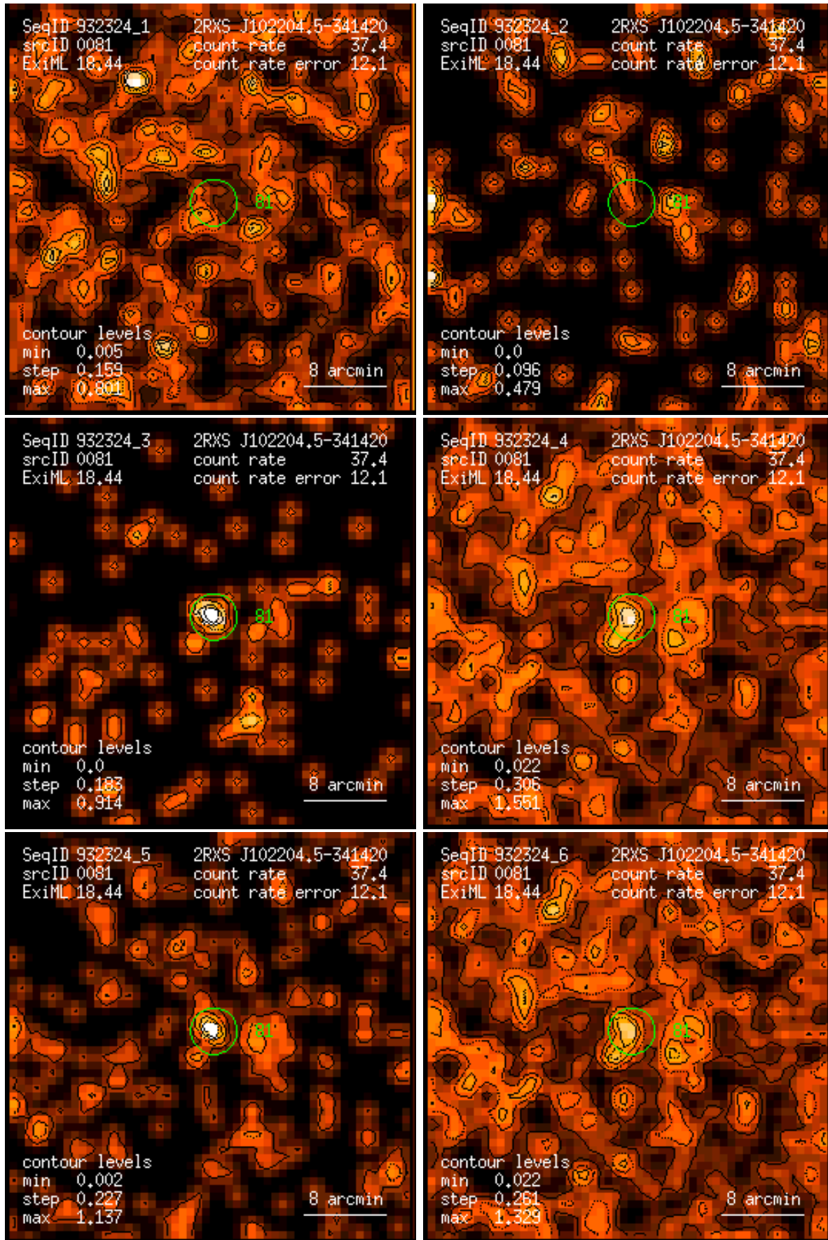
Figure 81: RASS 932324: detection 0081: band rate images, Gaussian filter: (1) PSPC channels 11 – 41, (2) 52 – 90, (3) 91 – 201, (4) 11 – 235, (5) 52 – 201, (6) 11 – 201. Broad band rates in counts/ks. Band rate contour levels in counts/ks/arcmin 2 .
