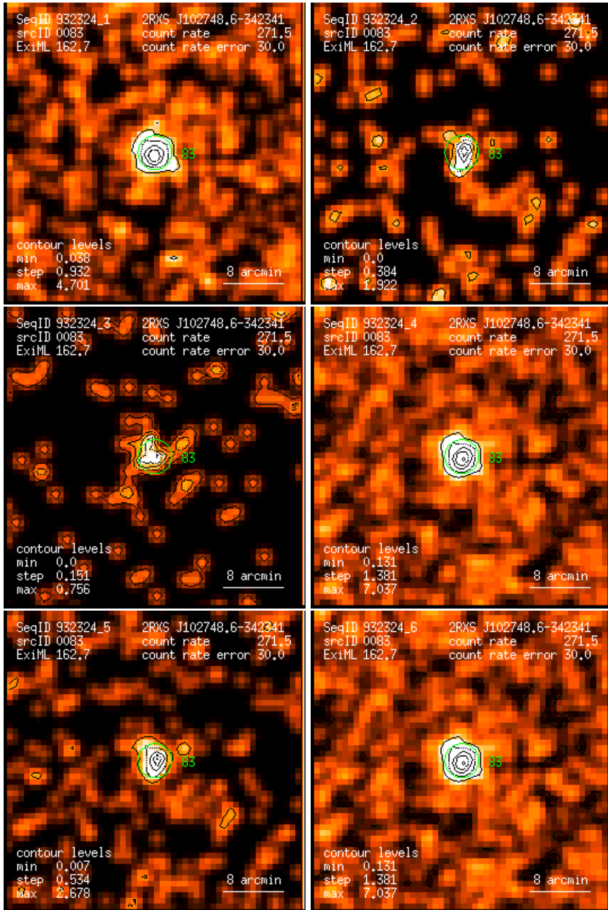
Figure 83: RASS 932324: detection 0083: band rate images, Gaussian filter: (1) PSPC channels 11 – 41, (2) 52 – 90, (3) 91 – 201, (4) 11 – 235, (5) 52 – 201, (6) 11 – 201. Broad band rates in counts/ks. Band rate contour levels in counts/ks/arcmin 2 .
