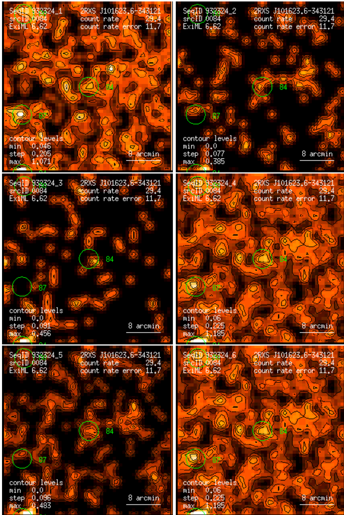
Figure 84: RASS 932324: detection 0084: band rate images, Gaussian filter: (1) PSPC channels 11 – 41, (2) 52 – 90, (3) 91 – 201, (4) 11 – 235, (5) 52 – 201, (6) 11 – 201. Broad band rates in counts/ks. Band rate contour levels in counts/ks/arcmin 2 .
