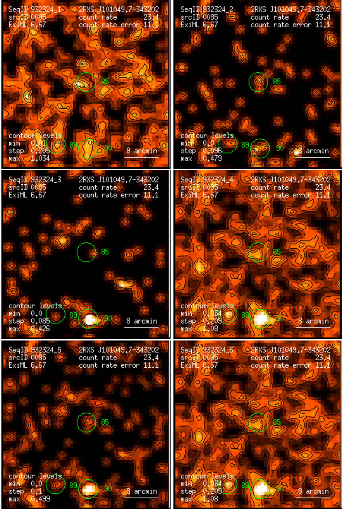
Figure 85: RASS 932324: detection 0085: band rate images, Gaussian filter: (1) PSPC channels 11 – 41, (2) 52 – 90, (3) 91 – 201, (4) 11 – 235, (5) 52 – 201, (6) 11 – 201. Broad band rates in counts/ks. Band rate contour levels in counts/ks/arcmin 2 .
