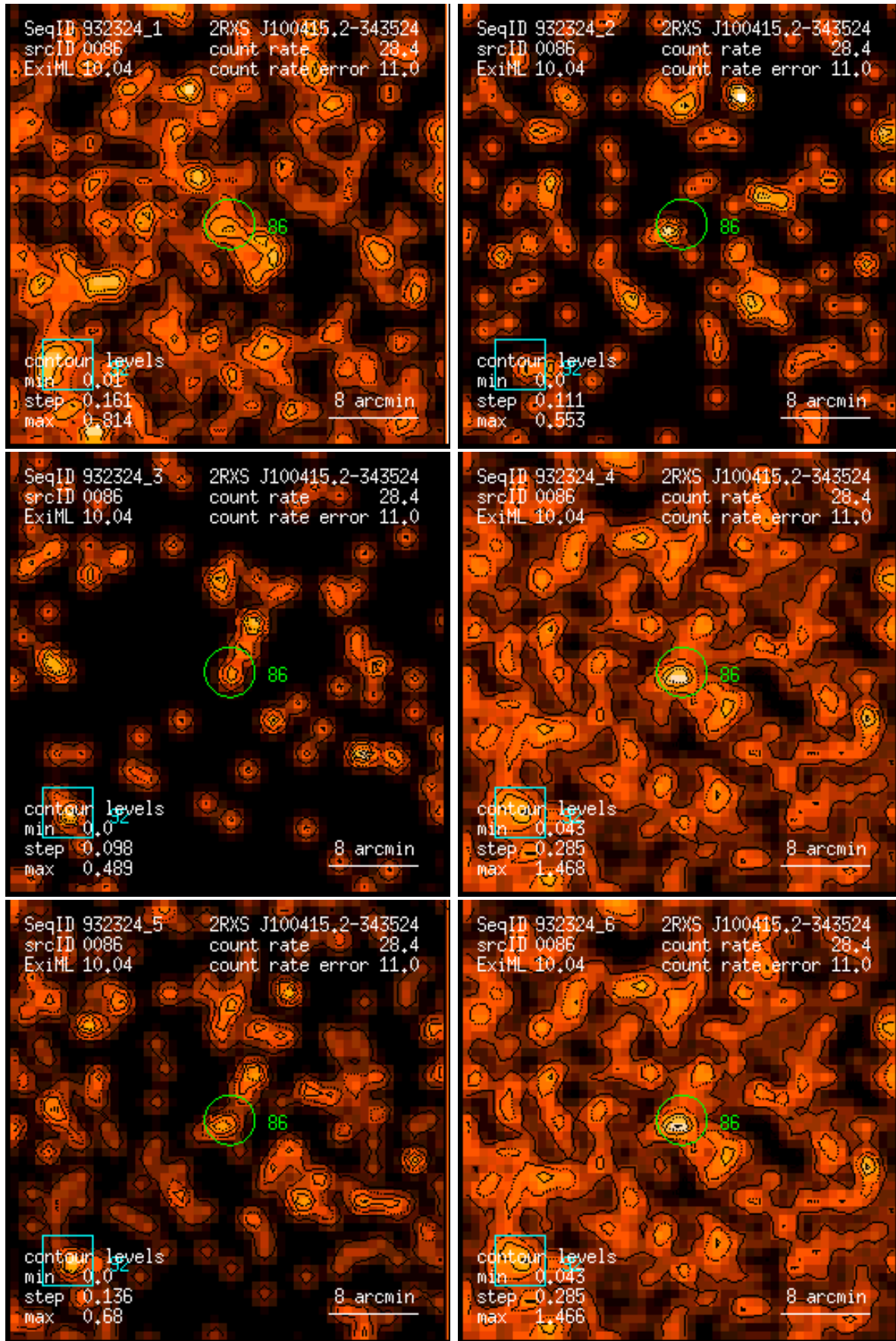
Figure 86: RASS 932324: detection 0086: band rate images, Gaussian filter: (1) PSPC channels 11 – 41, (2) 52 – 90, (3) 91 – 201, (4) 11 – 235, (5) 52 – 201, (6) 11 – 201. Broad band rates in counts/ks. Band rate contour levels in counts/ks/arcmin 2 .
