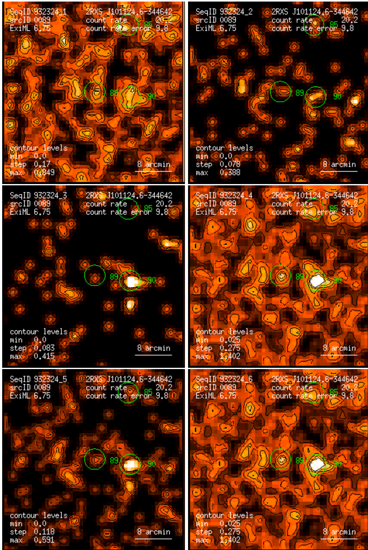
Figure 89: RASS 932324: detection 0089: band rate images, Gaussian filter: (1) PSPC channels 11 – 41, (2) 52 – 90, (3) 91 – 201, (4) 11 – 235, (5) 52 – 201, (6) 11 – 201. Broad band rates in counts/ks. Band rate contour levels in counts/ks/arcmin 2 .
