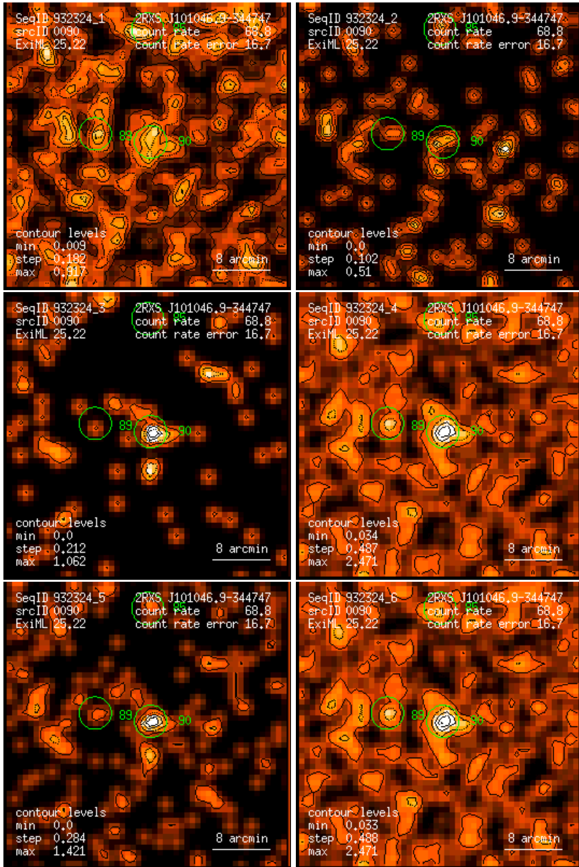
Figure 90: RASS 932324: detection 0090: band rate images, Gaussian filter: (1) PSPC channels 11 – 41, (2) 52 – 90, (3) 91 – 201, (4) 11 – 235, (5) 52 – 201, (6) 11 – 201. Broad band rates in counts/ks. Band rate contour levels in counts/ks/arcmin 2 .
