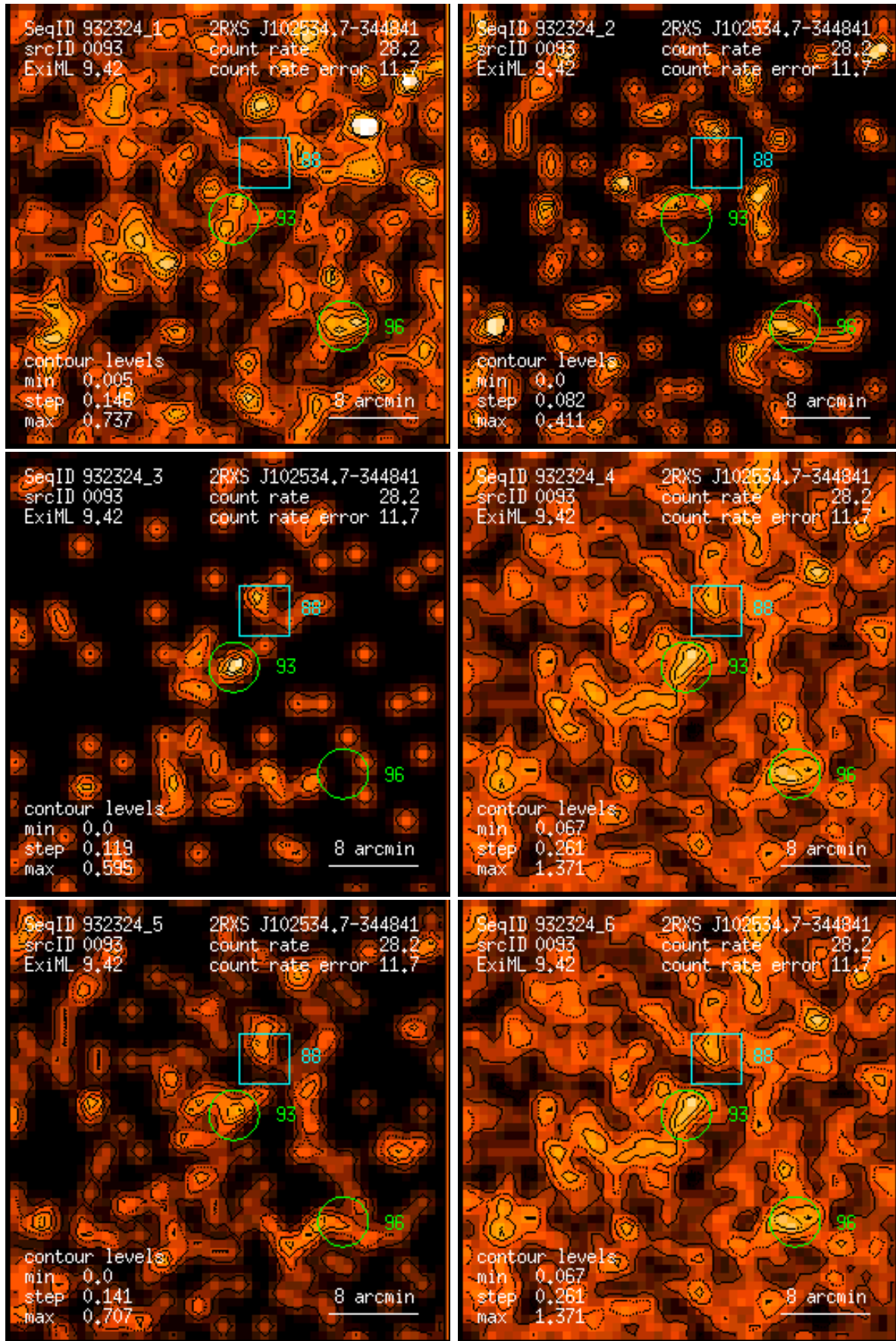
Figure 93: RASS 932324: detection 0093: band rate images, Gaussian filter: (1) PSPC channels 11 – 41, (2) 52 – 90, (3) 91 – 201, (4) 11 – 235, (5) 52 – 201, (6) 11 – 201. Broad band rates in counts/ks. Band rate contour levels in counts/ks/arcmin 2 .
