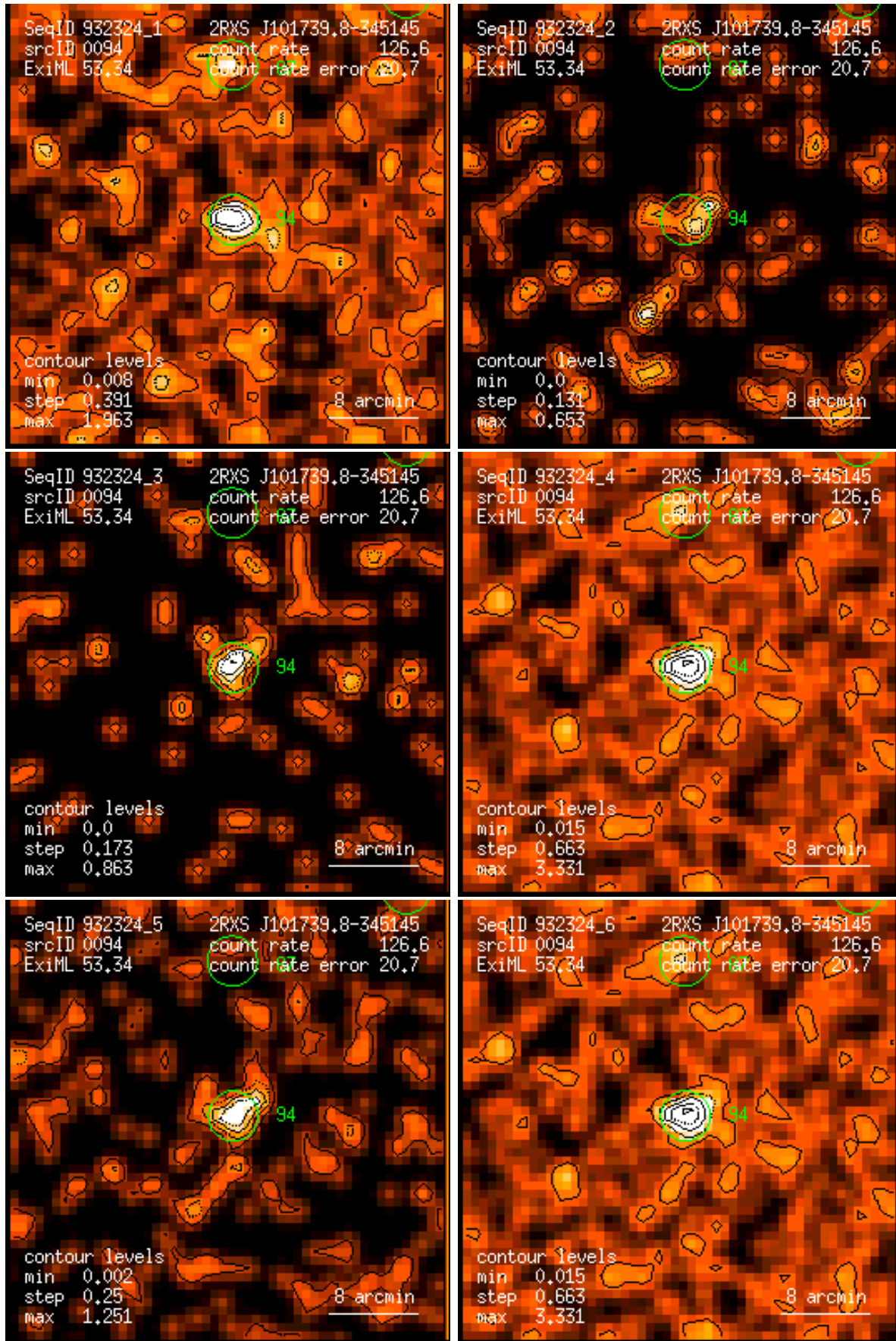
Figure 94: RASS 932324: detection 0094: band rate images, Gaussian filter: (1) PSPC channels 11 – 41, (2) 52 – 90, (3) 91 – 201, (4) 11 – 235, (5) 52 – 201, (6) 11 – 201. Broad band rates in counts/ks. Band rate contour levels in counts/ks/arcmin 2 .
