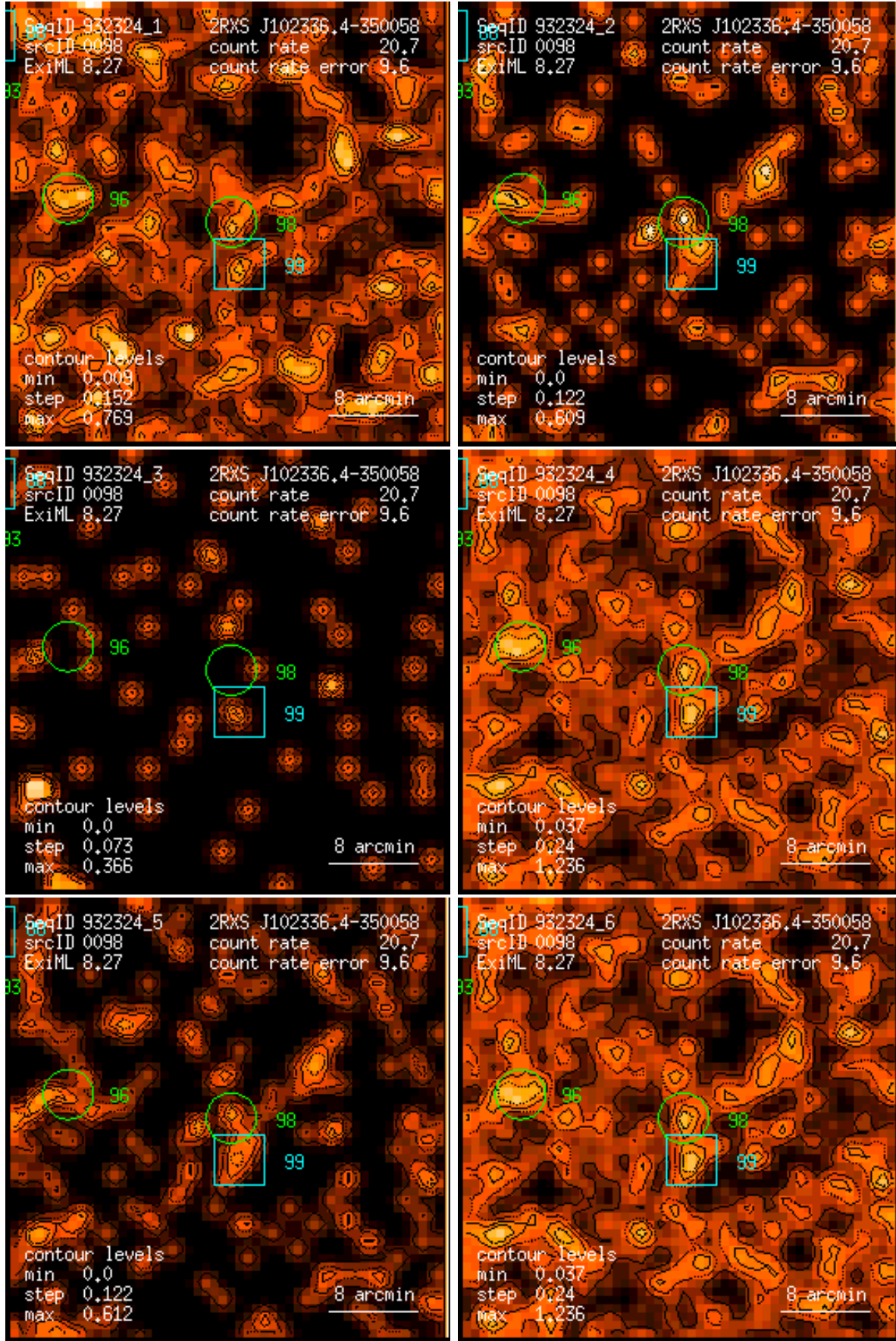
Figure 98: RASS 932324: detection 0098: band rate images, Gaussian filter: (1) PSPC channels 11 – 41, (2) 52 – 90, (3) 91 – 201, (4) 11 – 235, (5) 52 – 201, (6) 11 – 201. Broad band rates in counts/ks. Band rate contour levels in counts/ks/arcmin 2 .
