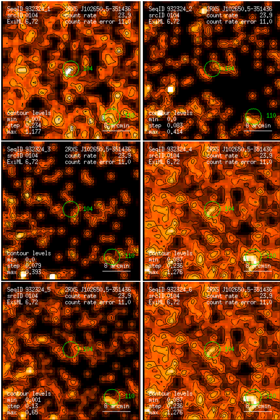
Figure 104: RASS 932324: detection 0104: band rate images, Gaussian filter: (1) PSPC channels 11 – 41, (2) 52 – 90, (3) 91 – 201, (4) 11 – 235, (5) 52 – 201, (6) 11 – 201. Broad band rates in counts/ks. Band rate contour levels in counts/ks/arcmin 2 .
