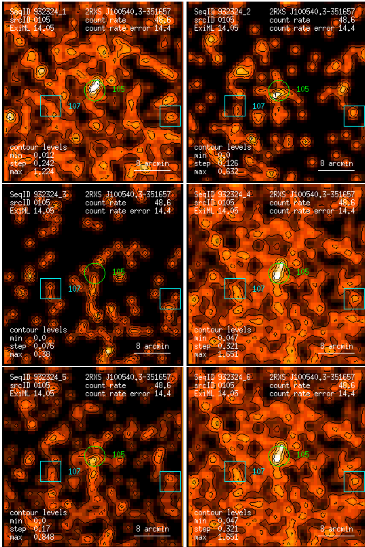
Figure 105: RASS 932324: detection 0105: band rate images, Gaussian filter: (1) PSPC channels 11 – 41, (2) 52 – 90, (3) 91 – 201, (4) 11 – 235, (5) 52 – 201, (6) 11 – 201. Broad band rates in counts/ks. Band rate contour levels in counts/ks/arcmin 2 .
