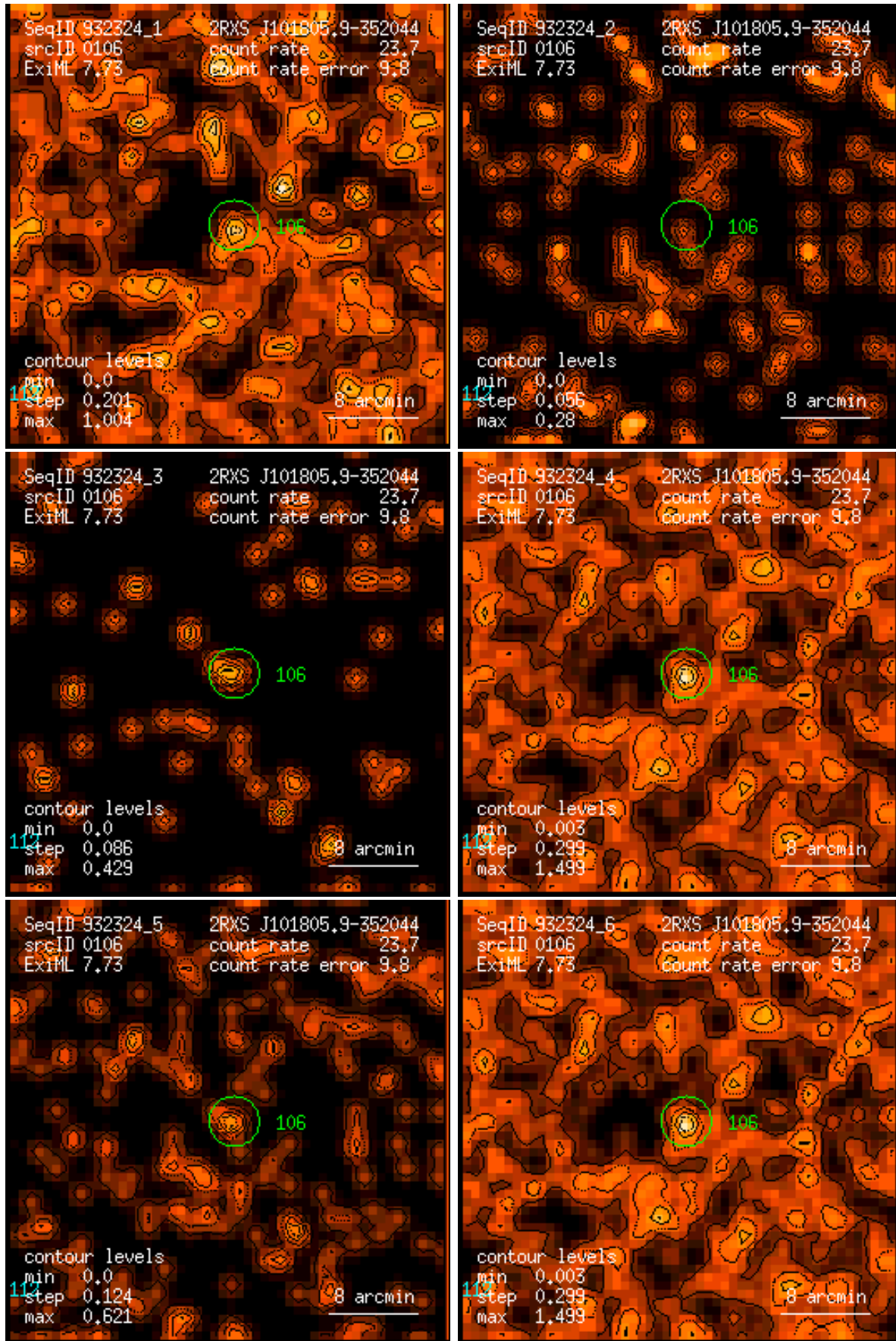
Figure 106: RASS 932324: detection 0106: band rate images, Gaussian filter: (1) PSPC channels 11 – 41, (2) 52 – 90, (3) 91 – 201, (4) 11 – 235, (5) 52 – 201, (6) 11 – 201. Broad band rates in counts/ks. Band rate contour levels in counts/ks/arcmin 2 .
