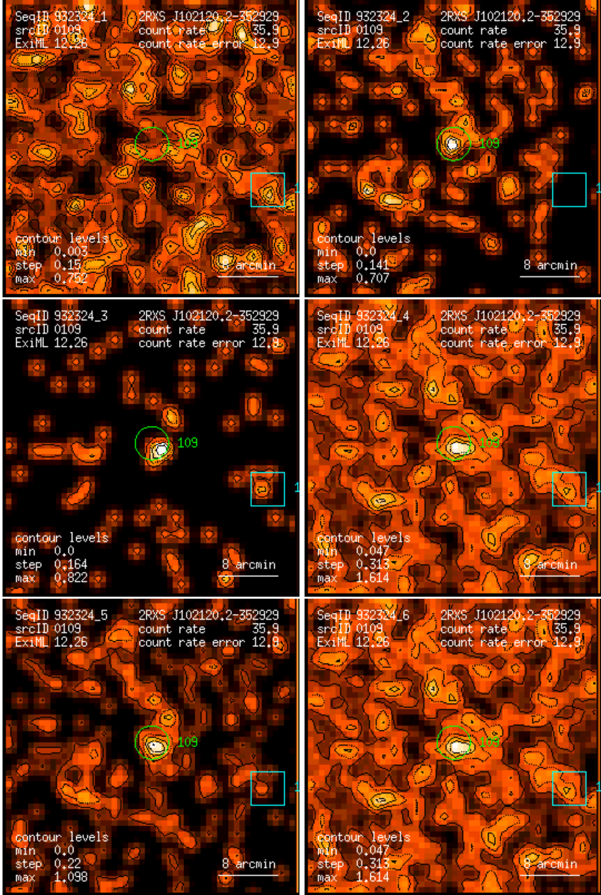
Figure 109: RASS 932324: detection 0109: band rate images, Gaussian filter: (1) PSPC channels 11 – 41, (2) 52 – 90, (3) 91 – 201, (4) 11 – 235, (5) 52 – 201, (6) 11 – 201. Broad band rates in counts/ks. Band rate contour levels in counts/ks/arcmin 2 .
