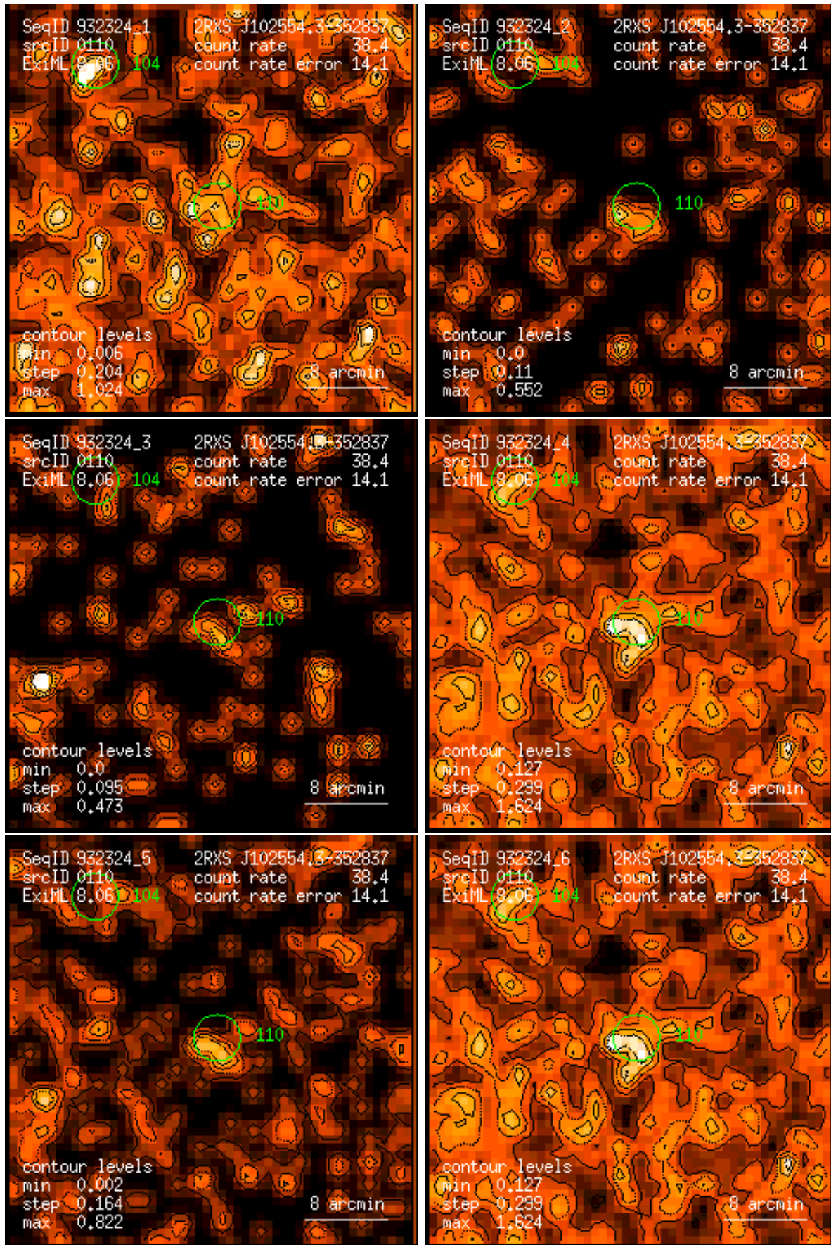
Figure 110: RASS 932324: detection 0110: band rate images, Gaussian filter: (1) PSPC channels 11 – 41, (2) 52 – 90, (3) 91 – 201, (4) 11 – 235, (5) 52 – 201, (6) 11 – 201. Broad band rates in counts/ks. Band rate contour levels in counts/ks/arcmin 2 .
