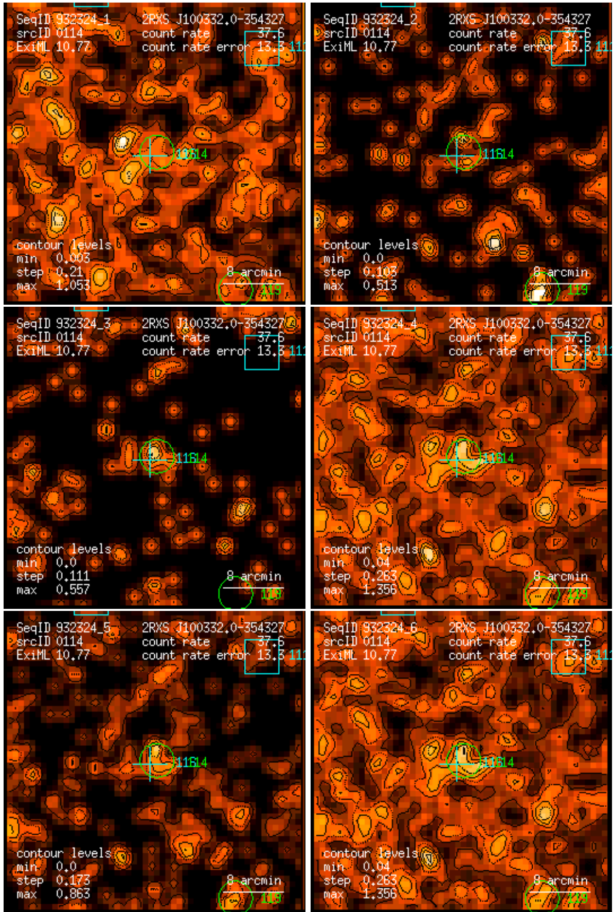
Figure 114: RASS 932324: detection 0114: band rate images, Gaussian filter: (1) PSPC channels 11 – 41, (2) 52 – 90, (3) 91 – 201, (4) 11 – 235, (5) 52 – 201, (6) 11 – 201. Broad band rates in counts/ks. Band rate contour levels in counts/ks/arcmin 2 .
