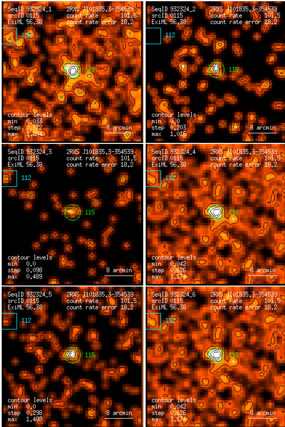
Figure 115: RASS 932324: detection 0115: band rate images, Gaussian filter: (1) PSPC channels 11 – 41, (2) 52 – 90, (3) 91 – 201, (4) 11 – 235, (5) 52 – 201, (6) 11 – 201. Broad band rates in counts/ks. Band rate contour levels in counts/ks/arcmin 2 .
