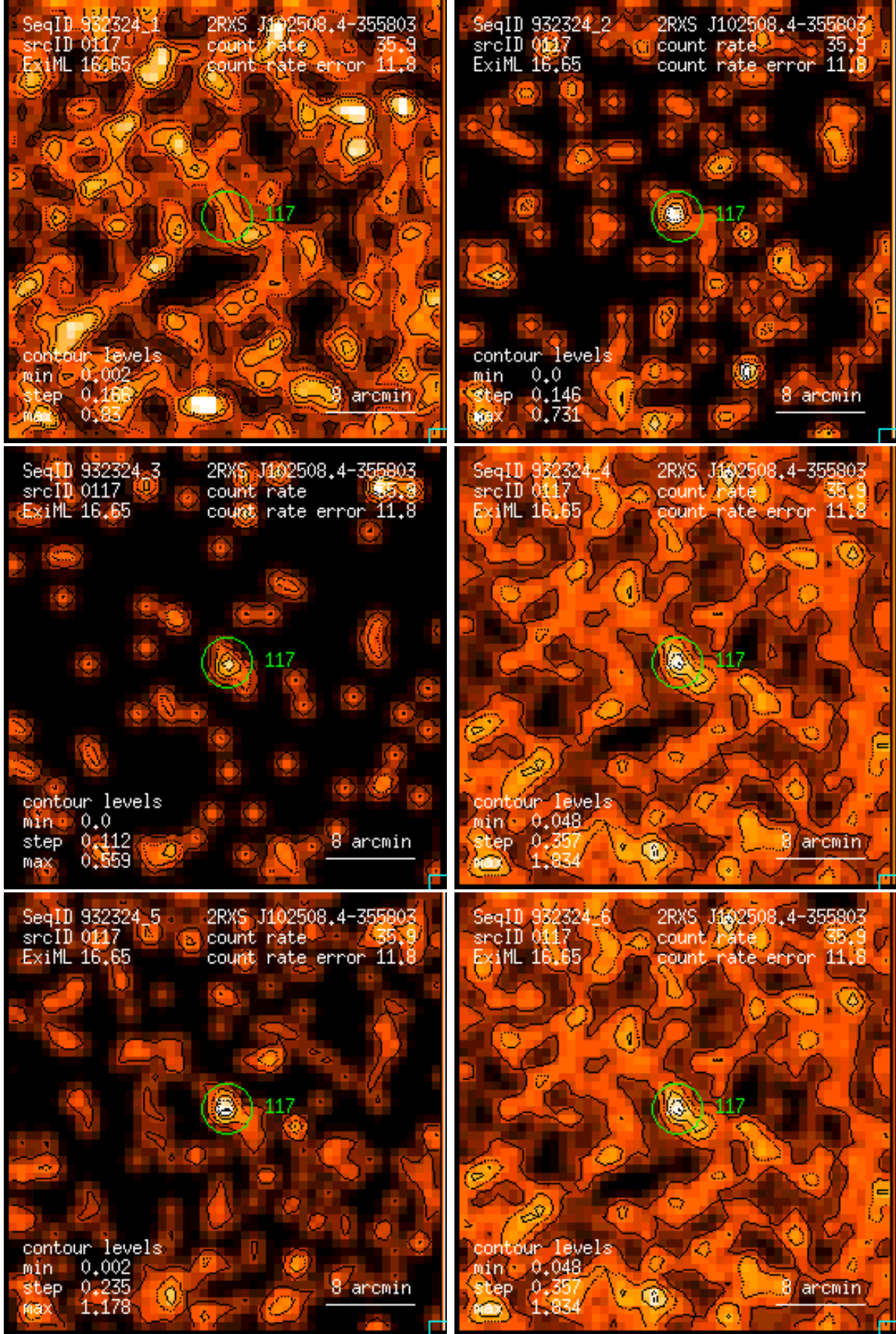
Figure 117: RASS 932324: detection 0117: band rate images, Gaussian filter: (1) PSPC channels 11 – 41, (2) 52 – 90, (3) 91 – 201, (4) 11 – 235, (5) 52 – 201, (6) 11 – 201. Broad band rates in counts/ks. Band rate contour levels in counts/ks/arcmin 2 .
