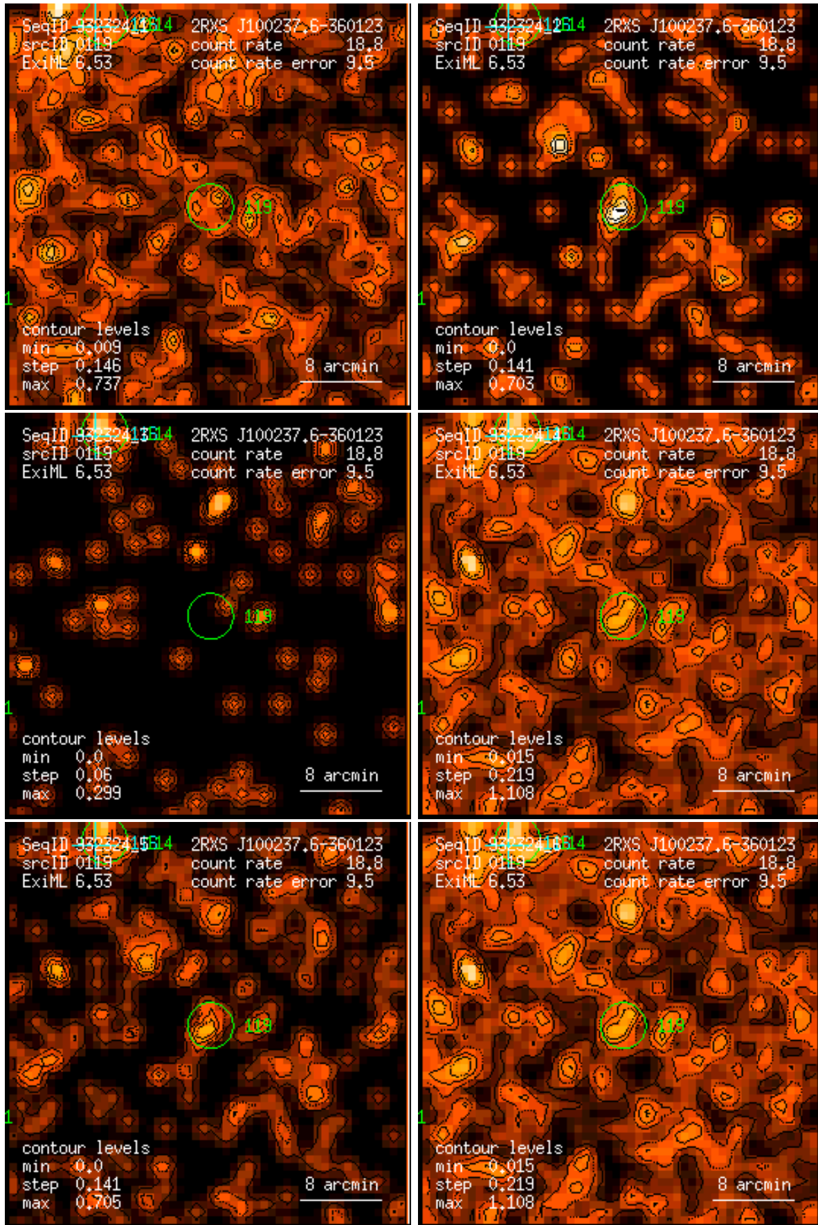
Figure 119: RASS 932324: detection 0119: band rate images, Gaussian filter: (1) PSPC channels 11 – 41, (2) 52 – 90, (3) 91 – 201, (4) 11 – 235, (5) 52 – 201, (6) 11 – 201. Broad band rates in counts/ks. Band rate contour levels in counts/ks/arcmin 2 .
