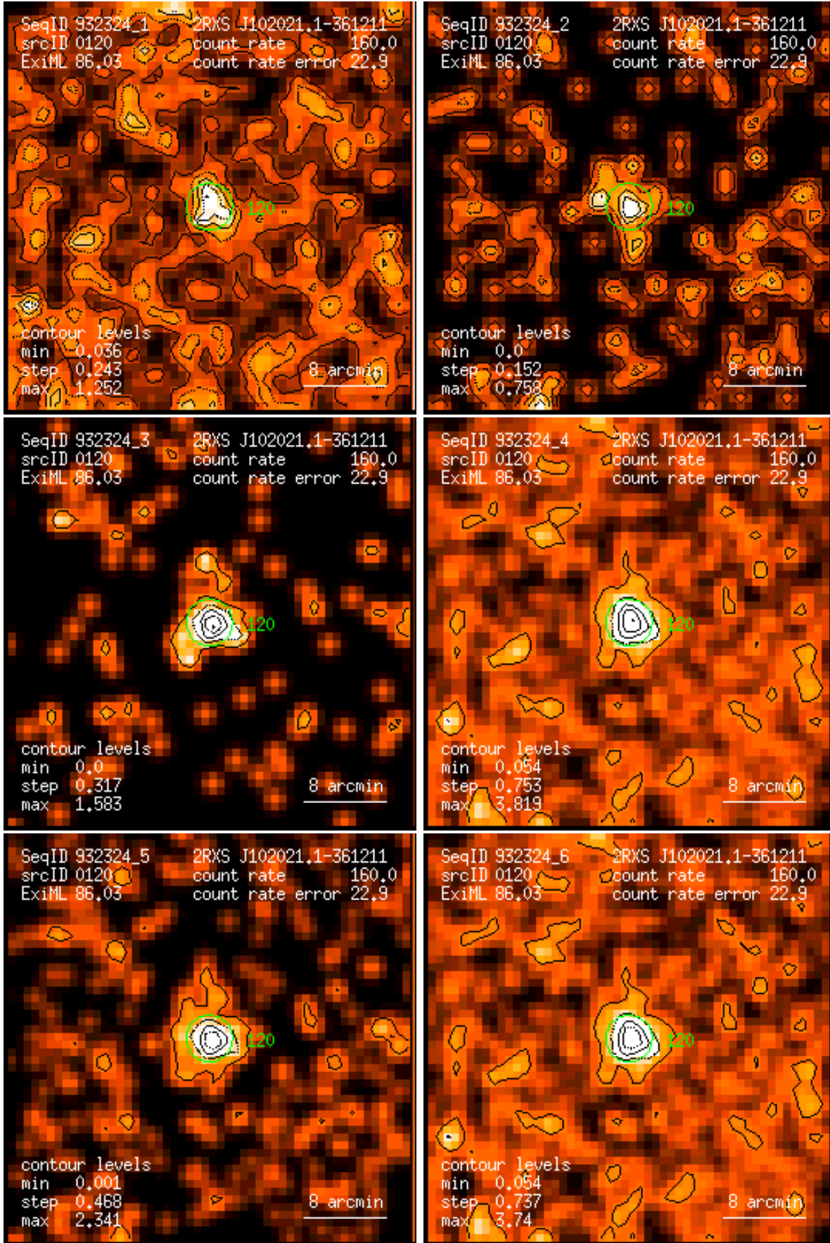
Figure 120: RASS 932324: detection 0120: band rate images, Gaussian filter: (1) PSPC channels 11 – 41, (2) 52 – 90, (3) 91 – 201, (4) 11 – 235, (5) 52 – 201, (6) 11 – 201. Broad band rates in counts/ks. Band rate contour levels in counts/ks/arcmin 2 .
