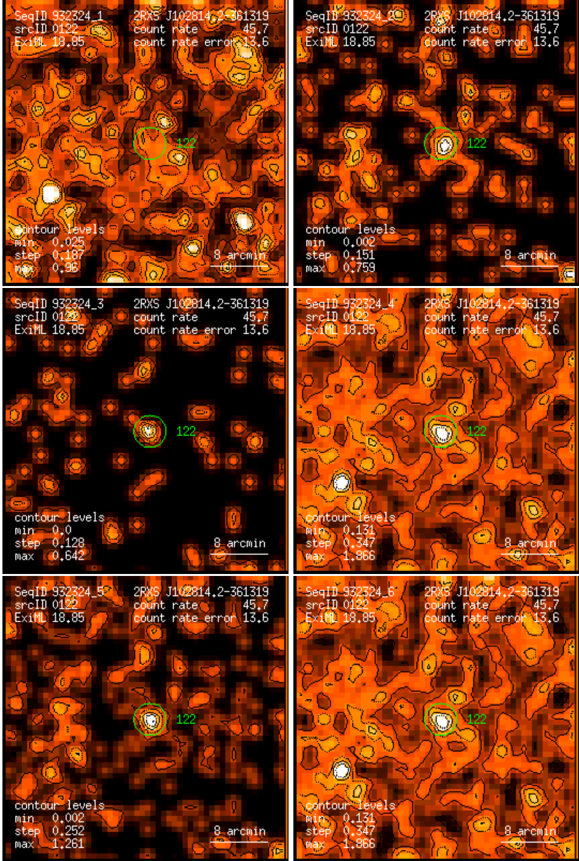
Figure 122: RASS 932324: detection 0122: band rate images, Gaussian filter: (1) PSPC channels 11 – 41, (2) 52 – 90, (3) 91 – 201, (4) 11 – 235, (5) 52 – 201, (6) 11 – 201. Broad band rates in counts/ks. Band rate contour levels in counts/ks/arcmin 2 .
