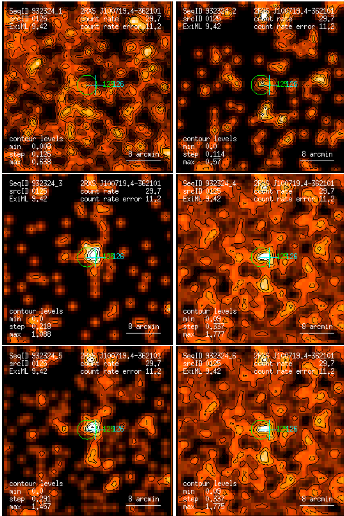
Figure 125: RASS 932324: detection 0125: band rate images, Gaussian filter: (1) PSPC channels 11 – 41, (2) 52 – 90, (3) 91 – 201, (4) 11 – 235, (5) 52 – 201, (6) 11 – 201. Broad band rates in counts/ks. Band rate contour levels in counts/ks/arcmin 2 .
