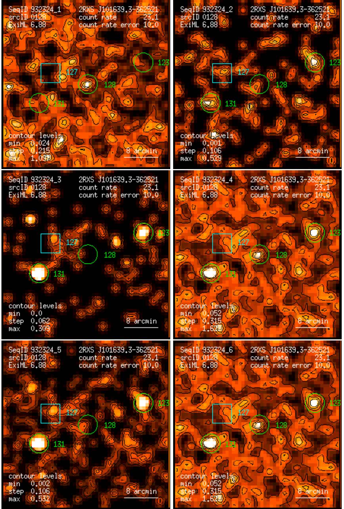
Figure 128: RASS 932324: detection 0128: band rate images, Gaussian filter: (1) PSPC channels 11 – 41, (2) 52 – 90, (3) 91 – 201, (4) 11 – 235, (5) 52 – 201, (6) 11 – 201. Broad band rates in counts/ks. Band rate contour levels in counts/ks/arcmin 2 .
