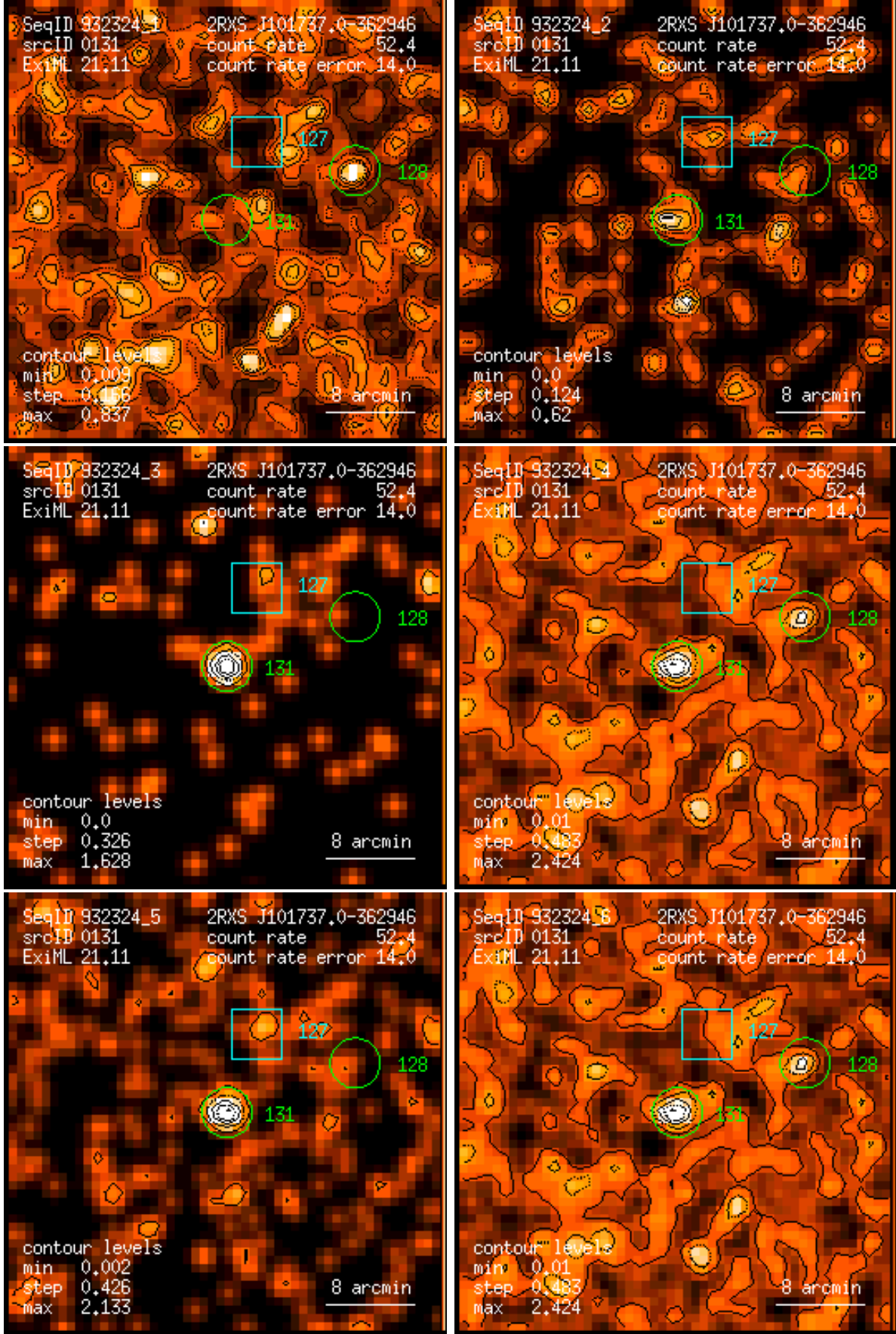
Figure 131: RASS 932324: detection 0131: band rate images, Gaussian filter: (1) PSPC channels 11 – 41, (2) 52 – 90, (3) 91 – 201, (4) 11 – 235, (5) 52 – 201, (6) 11 – 201. Broad band rates in counts/ks. Band rate contour levels in counts/ks/arcmin 2 .
