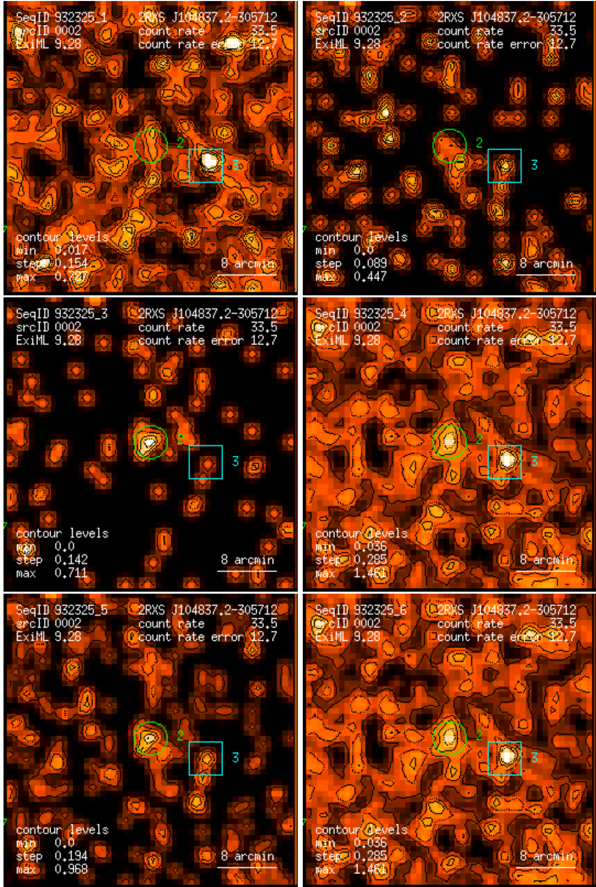
Figure 2: RASS 932325: detection 0002: band rate images, Gaussian filter: (1) PSPC channels 11 – 41, (2) 52 – 90, (3) 91 – 201, (4) 11 – 235, (5) 52 – 201, (6) 11 – 201. Broad band rates in counts/ks. Band rate contour levels in counts/ks/arcmin 2 .
