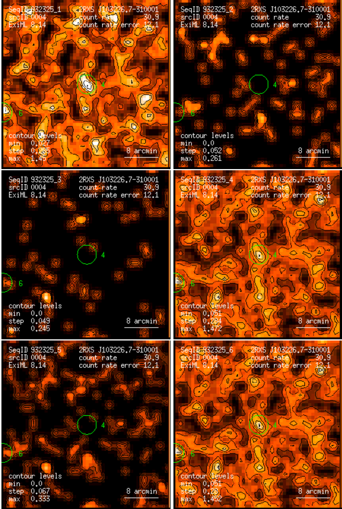
Figure 4: RASS 932325: detection 0004: band rate images, Gaussian filter: (1) PSPC channels 11 – 41, (2) 52 – 90, (3) 91 – 201, (4) 11 – 235, (5) 52 – 201, (6) 11 – 201. Broad band rates in counts/ks. Band rate contour levels in counts/ks/arcmin 2 .
