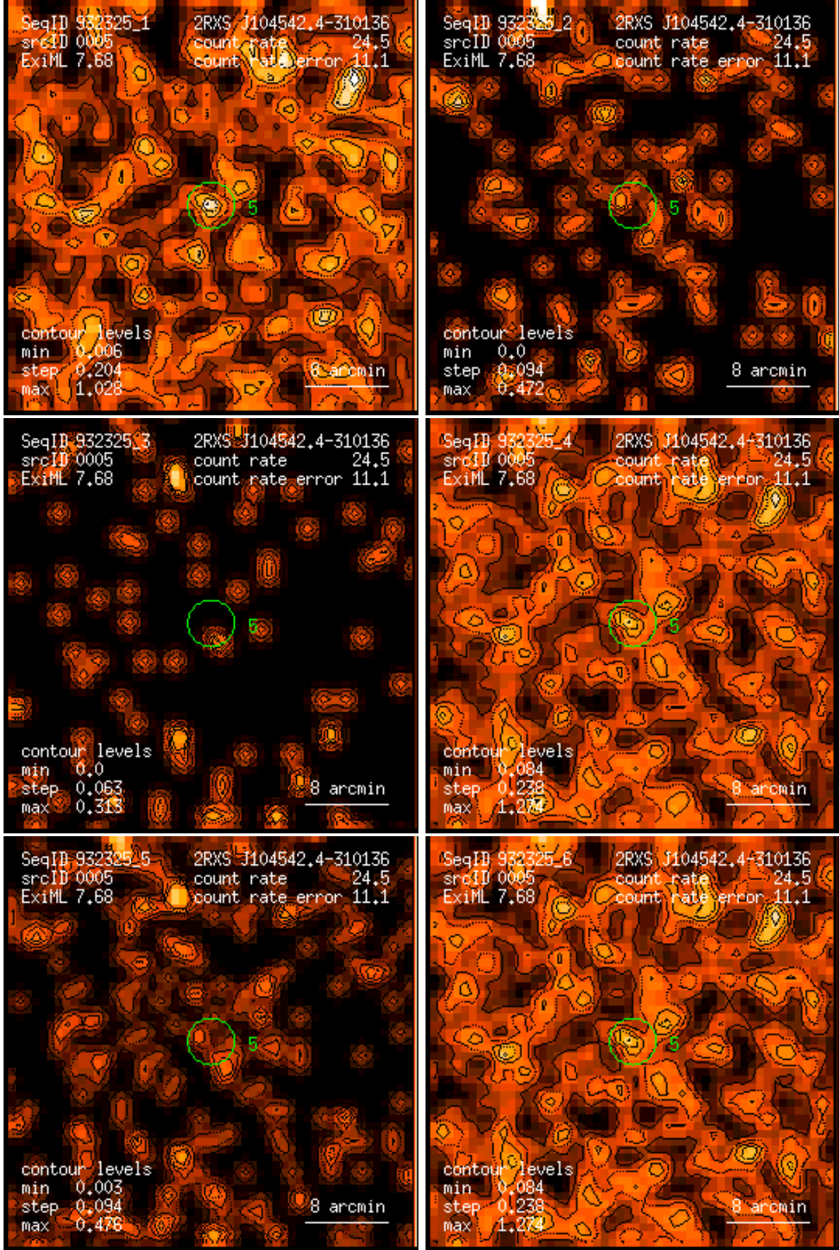
Figure 5: RASS 932325: detection 0005: band rate images, Gaussian filter: (1) PSPC channels 11 – 41, (2) 52 – 90, (3) 91 – 201, (4) 11 – 235, (5) 52 – 201, (6) 11 – 201. Broad band rates in counts/ks. Band rate contour levels in counts/ks/arcmin 2 .
