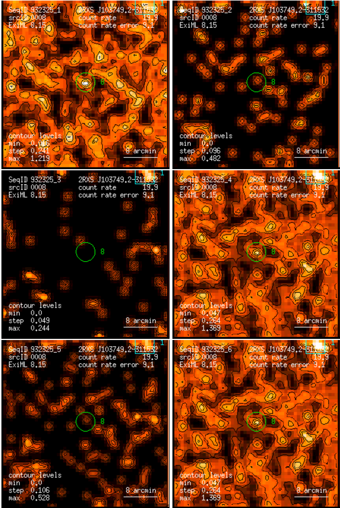
Figure 8: RASS 932325: detection 0008: band rate images, Gaussian filter: (1) PSPC channels 11 – 41, (2) 52 – 90, (3) 91 – 201, (4) 11 – 235, (5) 52 – 201, (6) 11 – 201. Broad band rates in counts/ks. Band rate contour levels in counts/ks/arcmin 2 .
