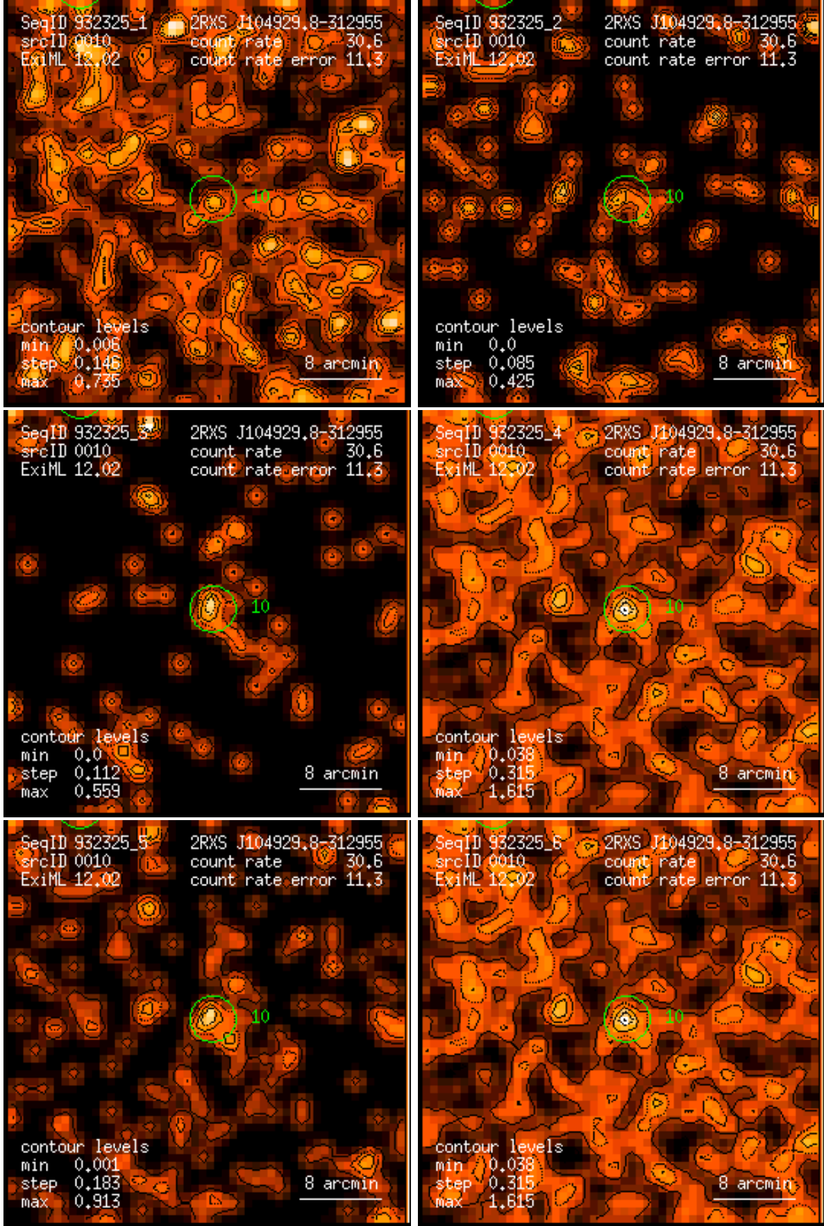
Figure 10: RASS 932325: detection 0010: band rate images, Gaussian filter: (1) PSPC channels 11 – 41, (2) 52 – 90, (3) 91 – 201, (4) 11 – 235, (5) 52 – 201, (6) 11 – 201. Broad band rates in counts/ks. Band rate contour levels in counts/ks/arcmin 2 .
