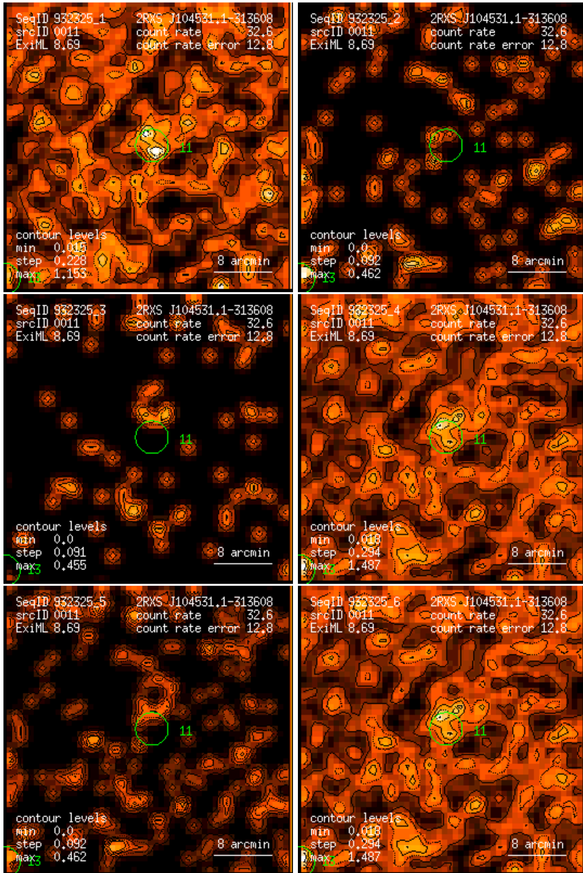
Figure 11: RASS 932325: detection 0011: band rate images, Gaussian filter: (1) PSPC channels 11 – 41, (2) 52 – 90, (3) 91 – 201, (4) 11 – 235, (5) 52 – 201, (6) 11 – 201. Broad band rates in counts/ks. Band rate contour levels in counts/ks/arcmin 2 .
