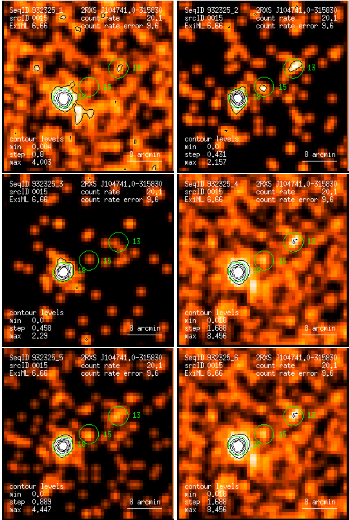
Figure 15: RASS 932325: detection 0015: band rate images, Gaussian filter: (1) PSPC channels 11 – 41, (2) 52 – 90, (3) 91 – 201, (4) 11 – 235, (5) 52 – 201, (6) 11 – 201. Broad band rates in counts/ks. Band rate contour levels in counts/ks/arcmin 2 .
