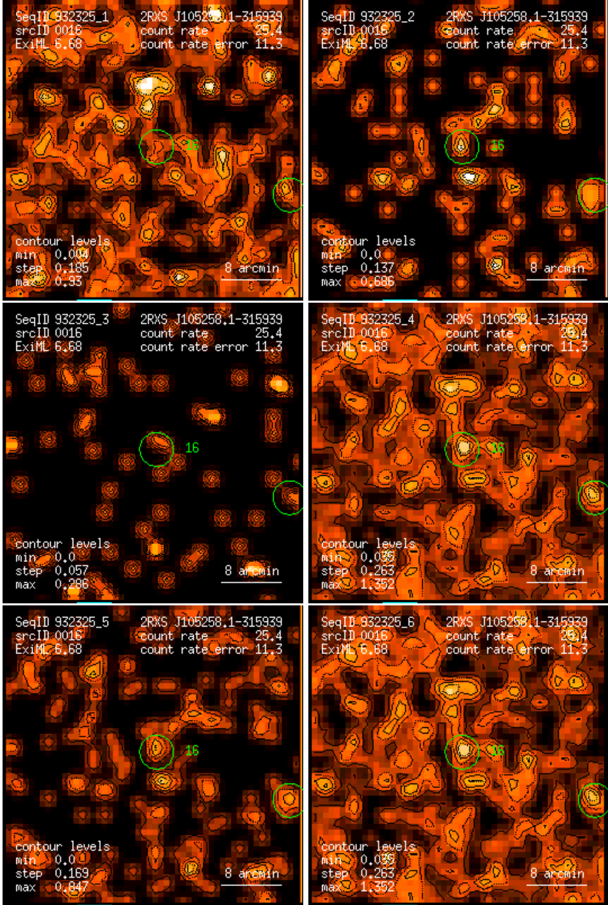
Figure 16: RASS 932325: detection 0016: band rate images, Gaussian filter: (1) PSPC channels 11 – 41, (2) 52 – 90, (3) 91 – 201, (4) 11 – 235, (5) 52 – 201, (6) 11 – 201. Broad band rates in counts/ks. Band rate contour levels in counts/ks/arcmin 2 .
