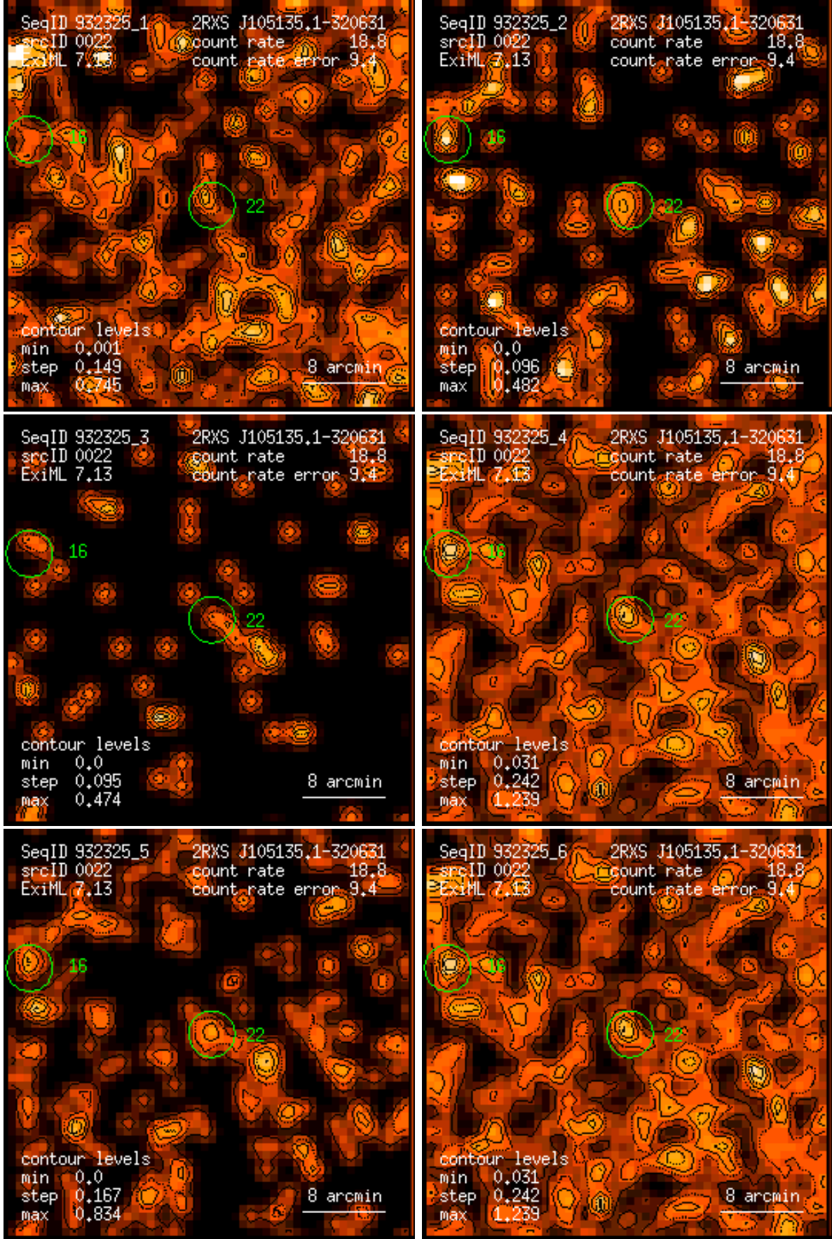
Figure 22: RASS 932325: detection 0022: band rate images, Gaussian filter: (1) PSPC channels 11 – 41, (2) 52 – 90, (3) 91 – 201, (4) 11 – 235, (5) 52 – 201, (6) 11 – 201. Broad band rates in counts/ks. Band rate contour levels in counts/ks/arcmin 2 .
