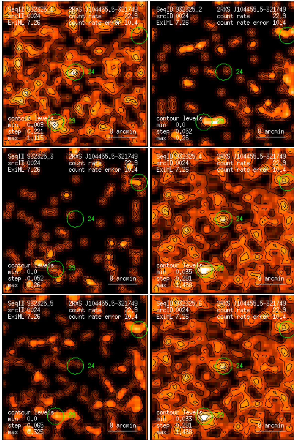
Figure 24: RASS 932325: detection 0024: band rate images, Gaussian filter: (1) PSPC channels 11 – 41, (2) 52 – 90, (3) 91 – 201, (4) 11 – 235, (5) 52 – 201, (6) 11 – 201. Broad band rates in counts/ks. Band rate contour levels in counts/ks/arcmin 2 .
