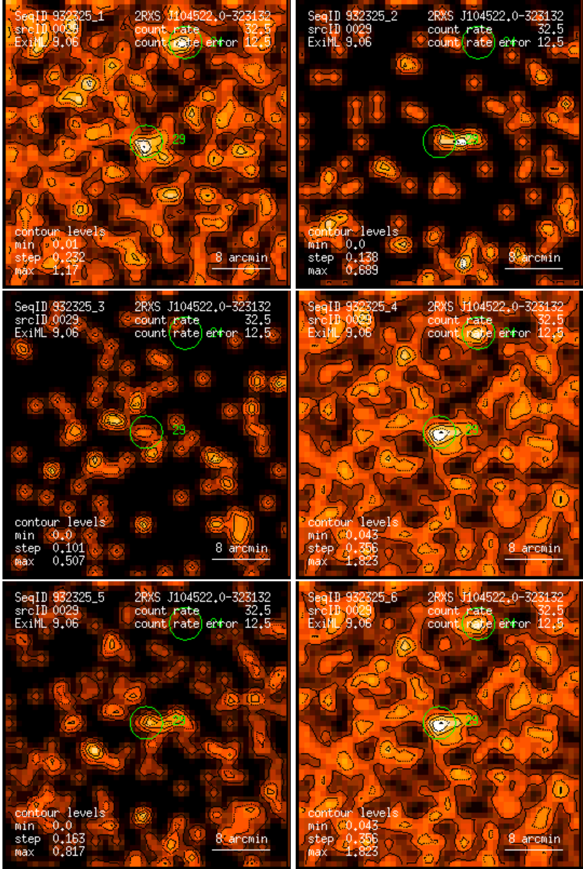
Figure 29: RASS 932325: detection 0029: band rate images, Gaussian filter: (1) PSPC channels 11 – 41, (2) 52 – 90, (3) 91 – 201, (4) 11 – 235, (5) 52 – 201, (6) 11 – 201. Broad band rates in counts/ks. Band rate contour levels in counts/ks/arcmin 2 .
