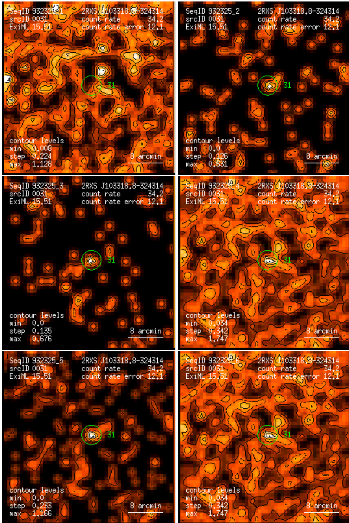
Figure 31: RASS 932325: detection 0031: band rate images, Gaussian filter: (1) PSPC channels 11 – 41, (2) 52 – 90, (3) 91 – 201, (4) 11 – 235, (5) 52 – 201, (6) 11 – 201. Broad band rates in counts/ks. Band rate contour levels in counts/ks/arcmin 2 .
