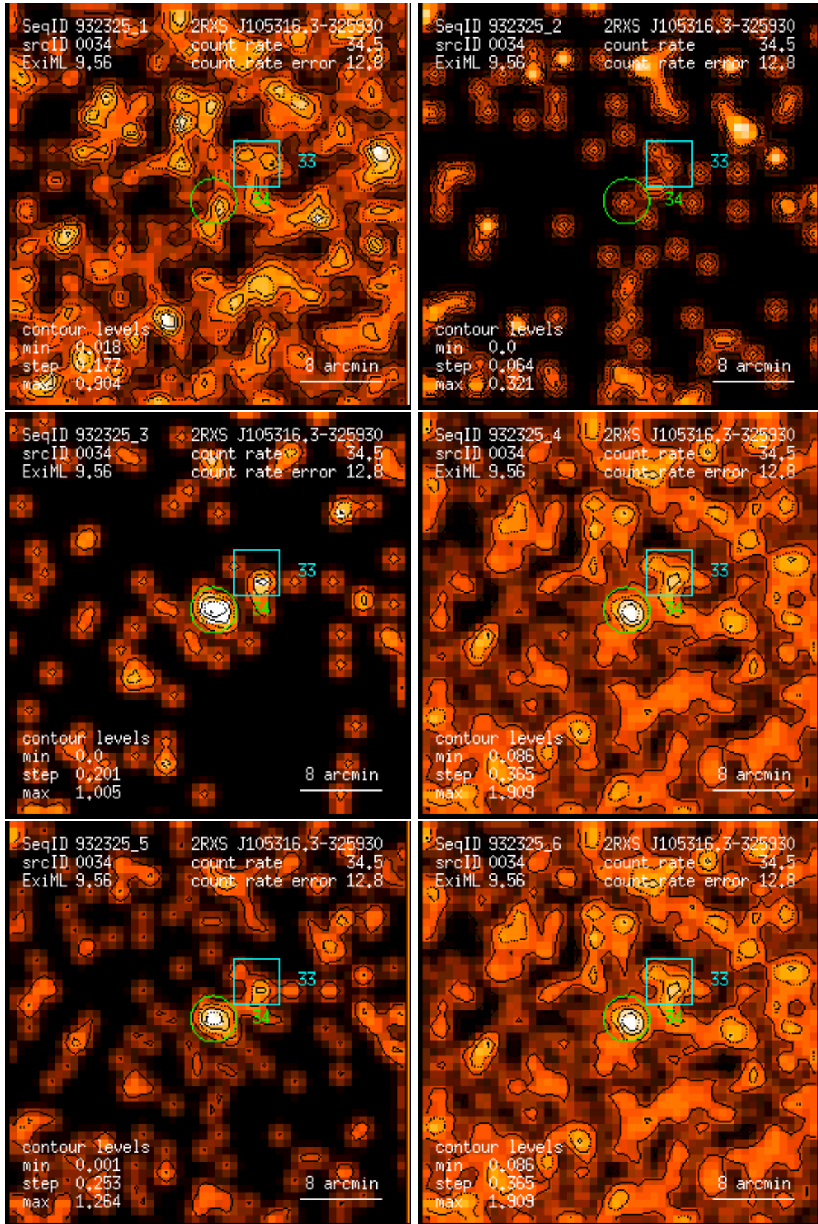
Figure 34: RASS 932325: detection 0034: band rate images, Gaussian filter: (1) PSPC channels 11 – 41, (2) 52 – 90, (3) 91 – 201, (4) 11 – 235, (5) 52 – 201, (6) 11 – 201. Broad band rates in counts/ks. Band rate contour levels in counts/ks/arcmin 2 .
