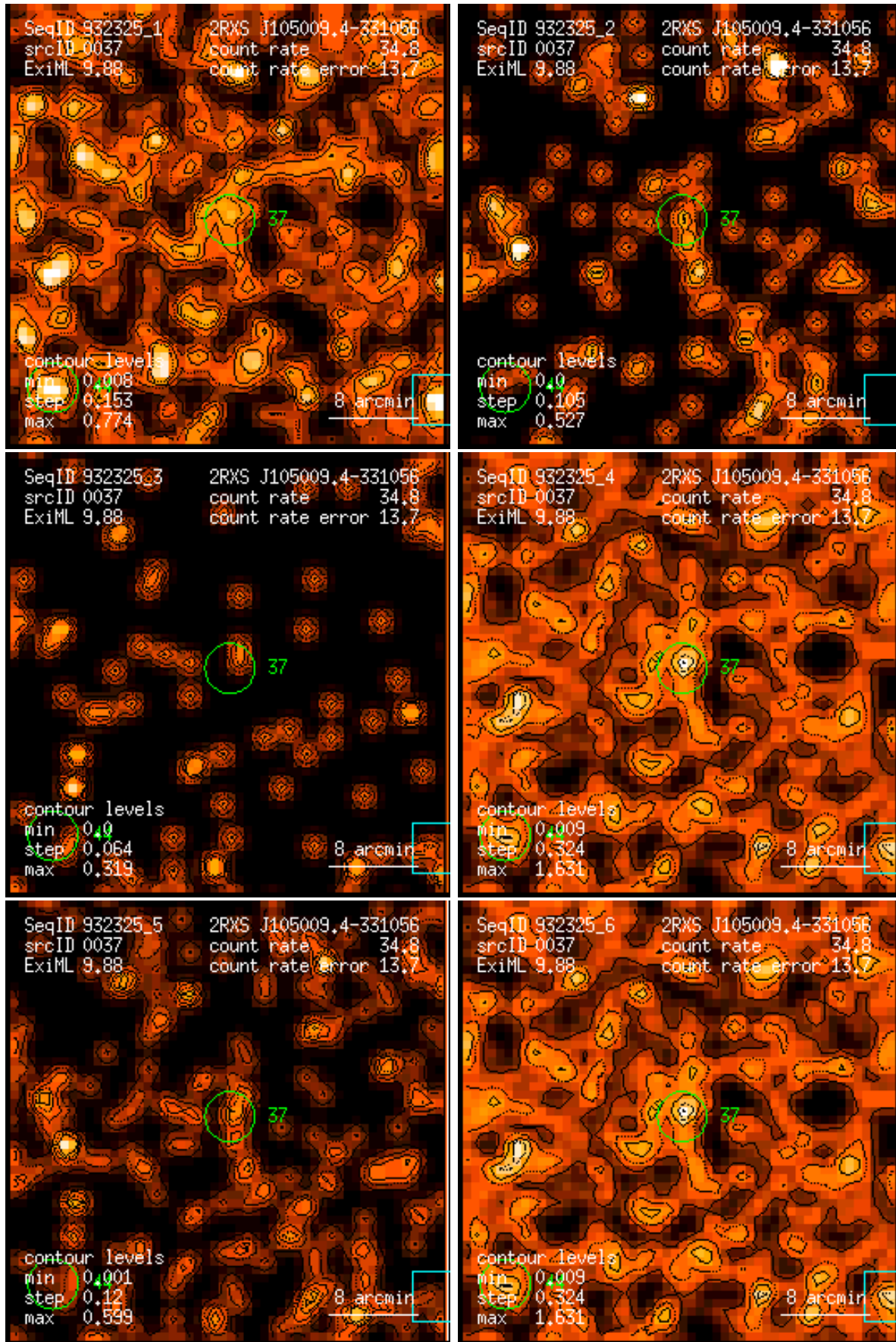
Figure 37: RASS 932325: detection 0037: band rate images, Gaussian filter: (1) PSPC channels 11 – 41, (2) 52 – 90, (3) 91 – 201, (4) 11 – 235, (5) 52 – 201, (6) 11 – 201. Broad band rates in counts/ks. Band rate contour levels in counts/ks/arcmin 2 .
