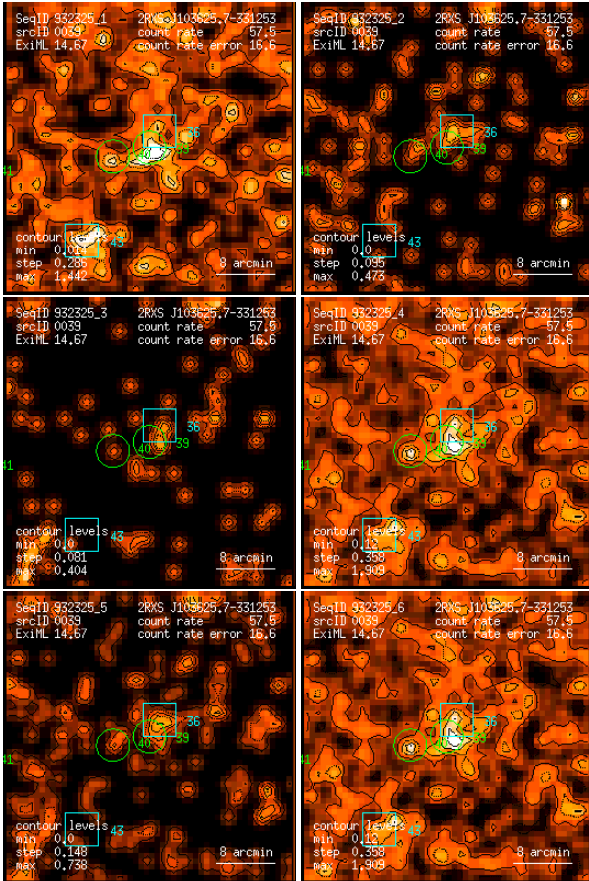
Figure 39: RASS 932325: detection 0039: band rate images, Gaussian filter: (1) PSPC channels 11 – 41, (2) 52 – 90, (3) 91 – 201, (4) 11 – 235, (5) 52 – 201, (6) 11 – 201. Broad band rates in counts/ks. Band rate contour levels in counts/ks/arcmin 2 .
