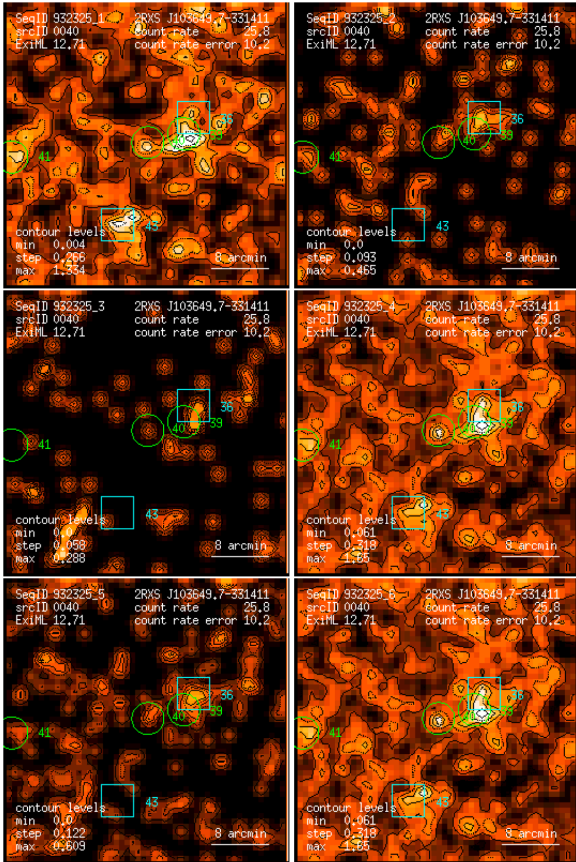
Figure 40: RASS 932325: detection 0040: band rate images, Gaussian filter: (1) PSPC channels 11 – 41, (2) 52 – 90, (3) 91 – 201, (4) 11 – 235, (5) 52 – 201, (6) 11 – 201. Broad band rates in counts/ks. Band rate contour levels in counts/ks/arcmin 2 .
