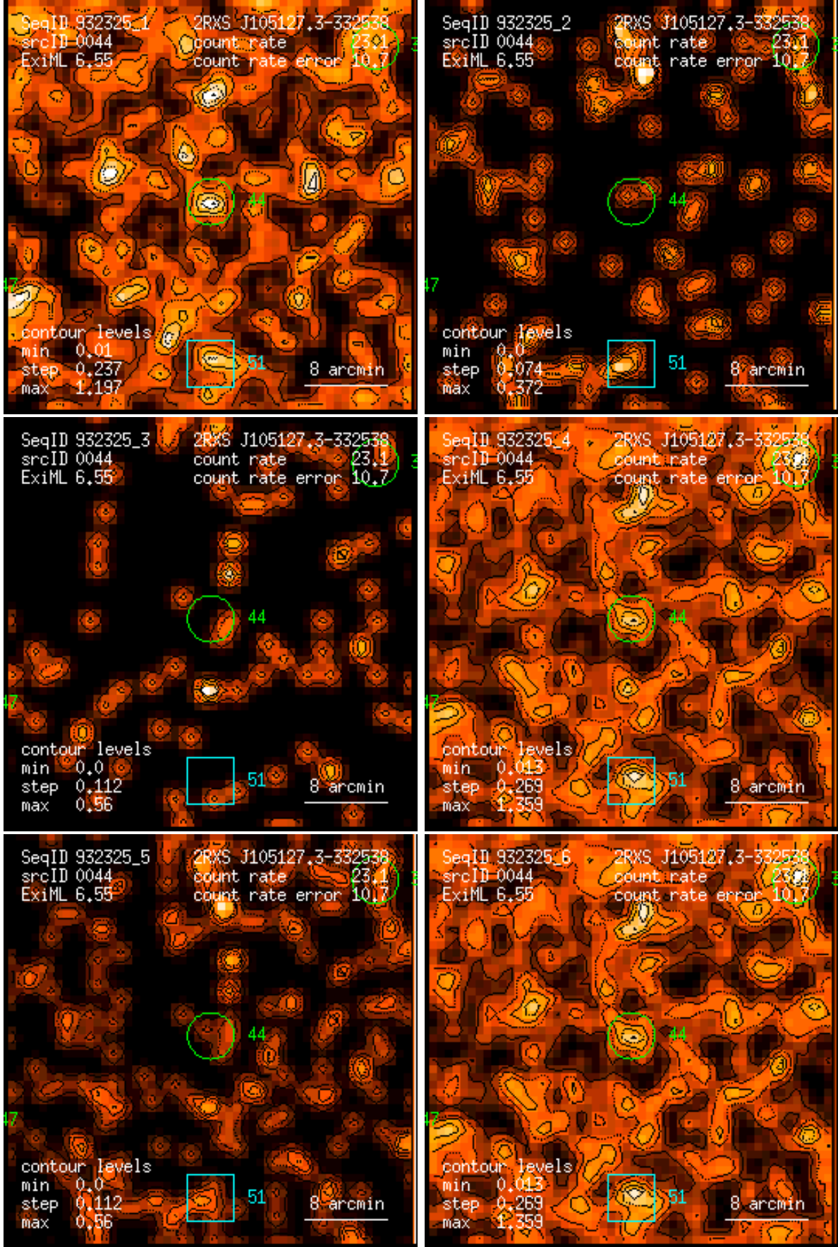
Figure 44: RASS 932325: detection 0044: band rate images, Gaussian filter: (1) PSPC channels 11 – 41, (2) 52 – 90, (3) 91 – 201, (4) 11 – 235, (5) 52 – 201, (6) 11 – 201. Broad band rates in counts/ks. Band rate contour levels in counts/ks/arcmin 2 .
