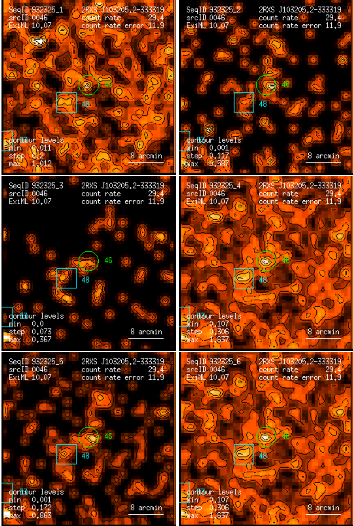
Figure 46: RASS 932325: detection 0046: band rate images, Gaussian filter: (1) PSPC channels 11 – 41, (2) 52 – 90, (3) 91 – 201, (4) 11 – 235, (5) 52 – 201, (6) 11 – 201. Broad band rates in counts/ks. Band rate contour levels in counts/ks/arcmin 2 .
