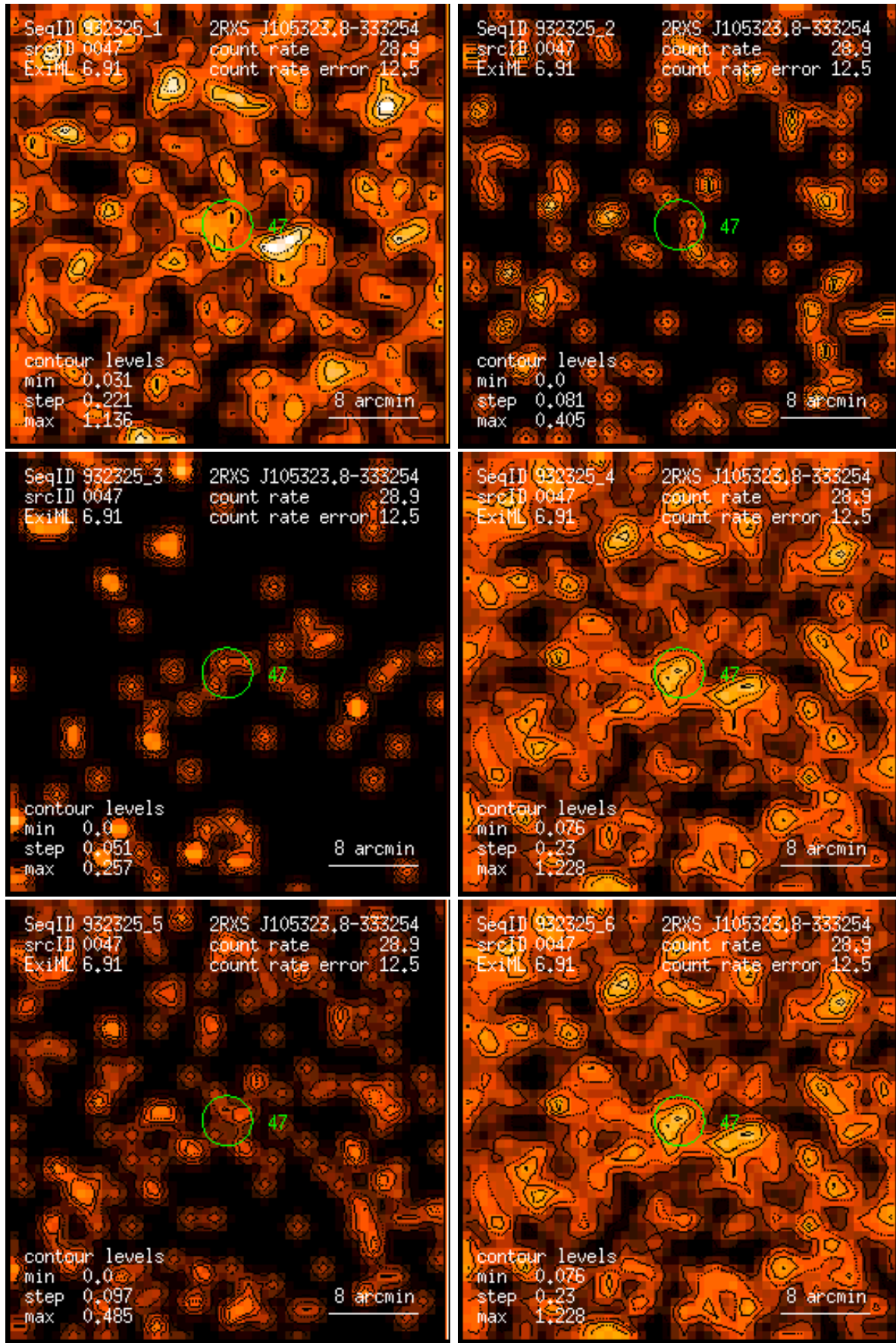
Figure 47: RASS 932325: detection 0047: band rate images, Gaussian filter: (1) PSPC channels 11 – 41, (2) 52 – 90, (3) 91 – 201, (4) 11 – 235, (5) 52 – 201, (6) 11 – 201. Broad band rates in counts/ks. Band rate contour levels in counts/ks/arcmin 2 .
