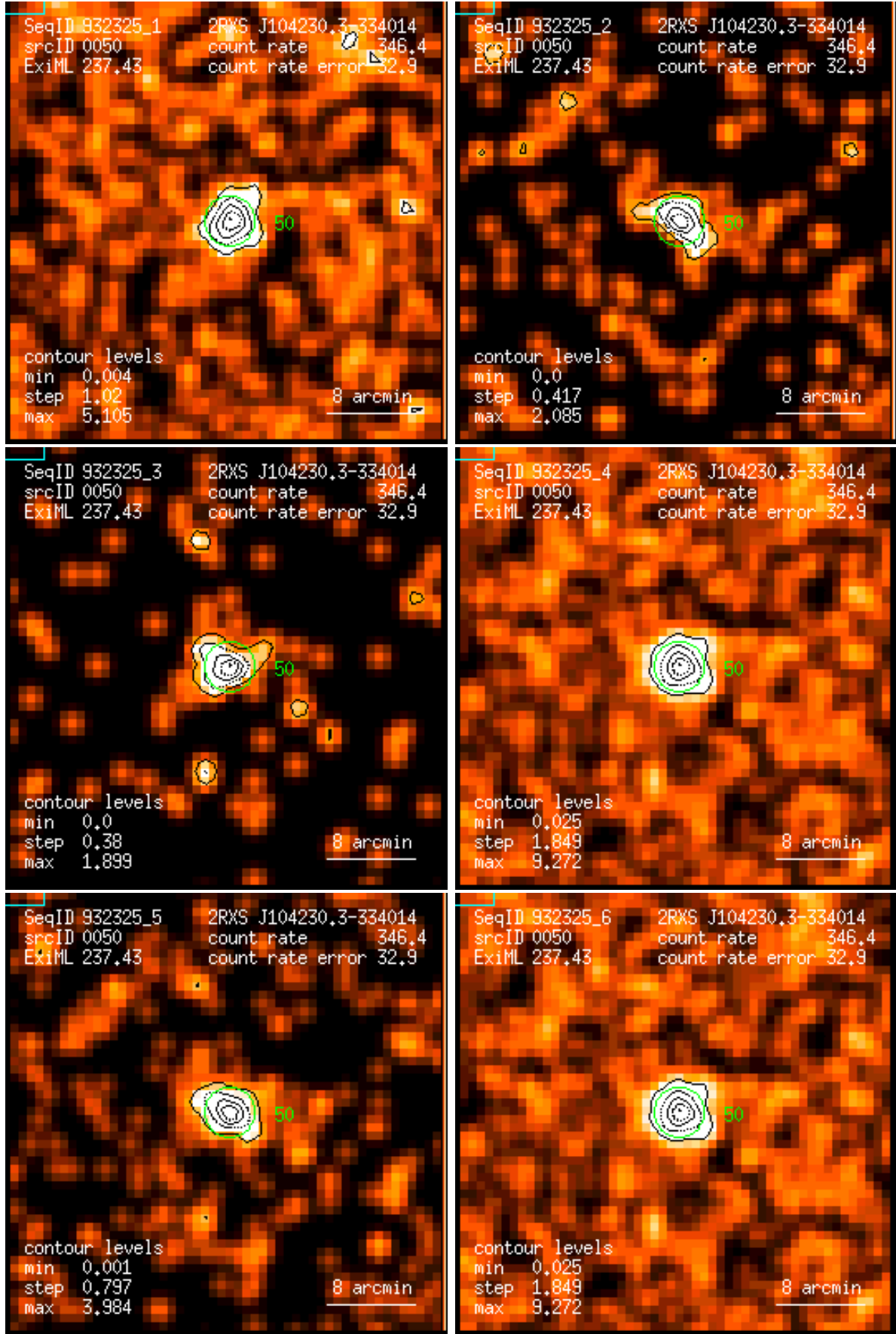
Figure 50: RASS 932325: detection 0050: band rate images, Gaussian filter: (1) PSPC channels 11 – 41, (2) 52 – 90, (3) 91 – 201, (4) 11 – 235, (5) 52 – 201, (6) 11 – 201. Broad band rates in counts/ks. Band rate contour levels in counts/ks/arcmin 2 .
