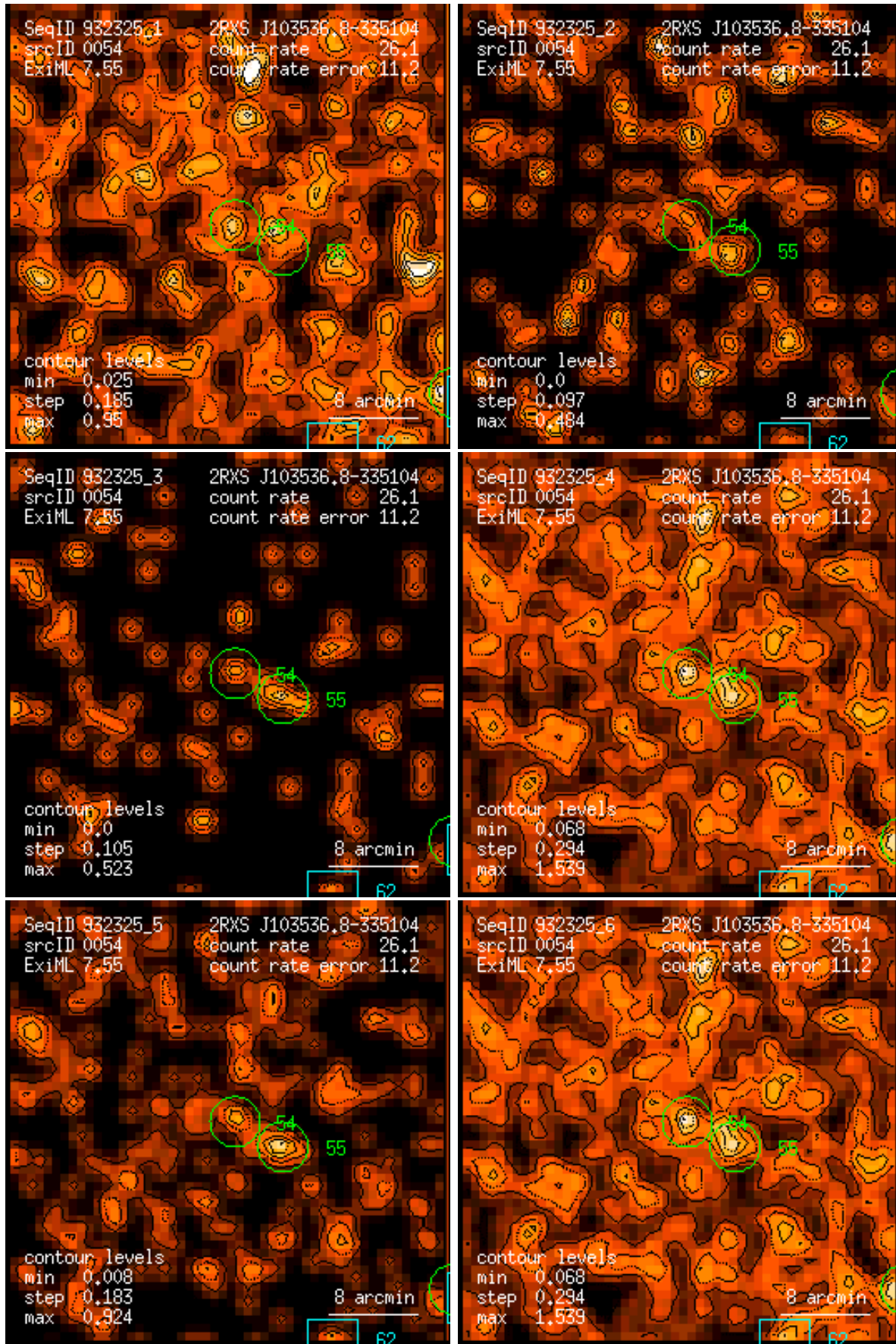
Figure 54: RASS 932325: detection 0054: band rate images, Gaussian filter: (1) PSPC channels 11 – 41, (2) 52 – 90, (3) 91 – 201, (4) 11 – 235, (5) 52 – 201, (6) 11 – 201. Broad band rates in counts/ks. Band rate contour levels in counts/ks/arcmin 2 .
