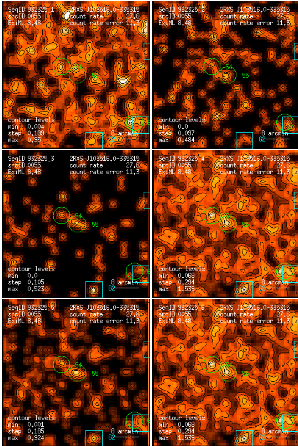
Figure 55: RASS 932325: detection 0055: band rate images, Gaussian filter: (1) PSPC channels 11 – 41, (2) 52 – 90, (3) 91 – 201, (4) 11 – 235, (5) 52 – 201, (6) 11 – 201. Broad band rates in counts/ks. Band rate contour levels in counts/ks/arcmin 2 .
